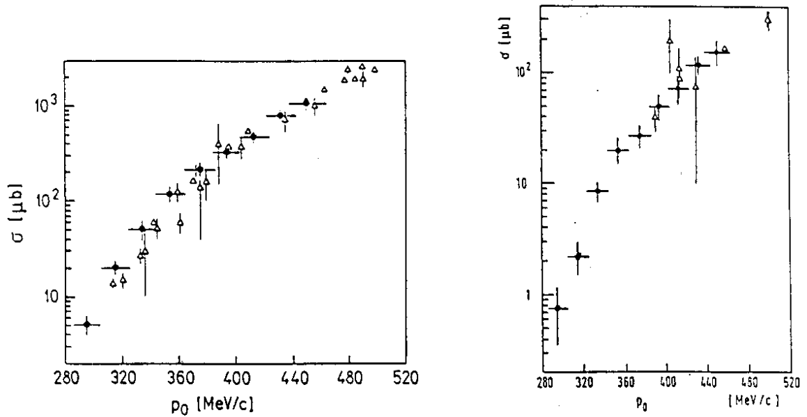
Figure 2: Integrated cross sections for \pi^-p \rightarrow \pi^+\pi^-n (left) and \pi^-p \rightarrow \pi^-\pi\pi^0 (right) as measured in this experiment (full circles) compared to previous experimental studies. Statistical and systematic errors have been summed in quadrature.
