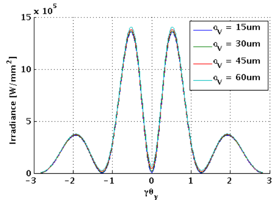
Figure 2: DR angular distribution for various beam sizes at 400 nm.
