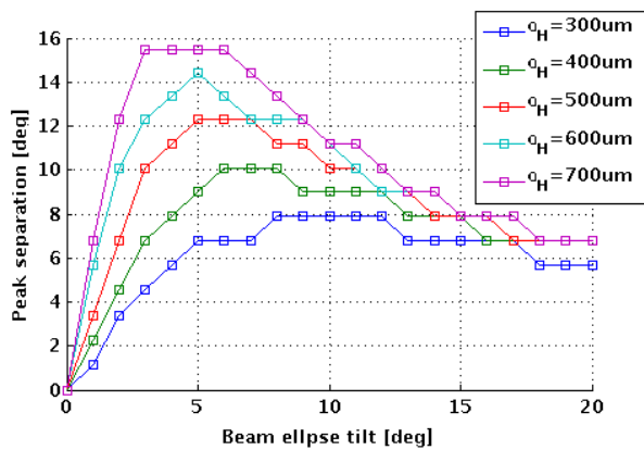
Figure 5: Peak separation between the left and right tine versus the input beam ellipse tilt for \lambda = 400 nm.
