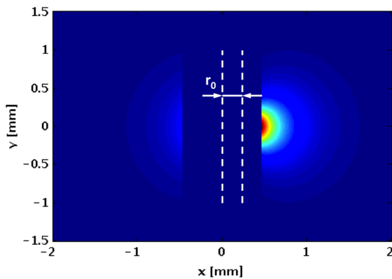
Figure 1: Source field for a single particle passing through a slit with an offset r_0 .
