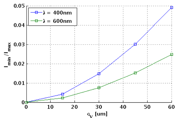
Figure 3: Simulated visibility versus beam size.
