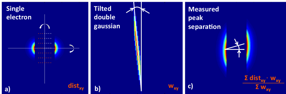
Figure 4: Imaged irradiance from a single electron (a), two-dimensional gaussian beam profile (b) and imaged irradiance from a two dimensional beam (c)
