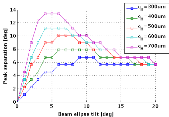
Figure 6: Peak separation between the left and right tine versus the input beam ellipse tilt for \lambda = 600 nm.
