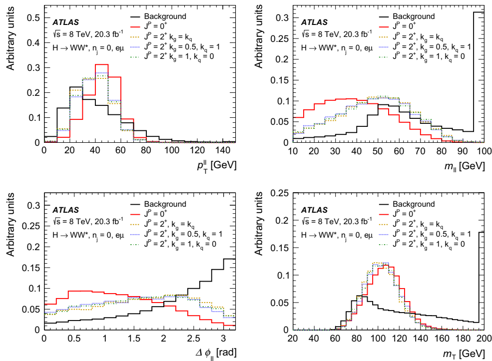
Fig. 2 Expected normalised Higgs-boson distributions of the transverse momentum of the dilepton system p_T^{\text{H}} , the dilepton mass m_{\ell\ell} , the azimuthal angular difference between the leptons \Delta\phi_{\ell\ell} and the transverse mass m_T for the e\mu+0 -jet category. The distributions are shown for the SM signal hypothesis (solid red line) and for three spin-2
