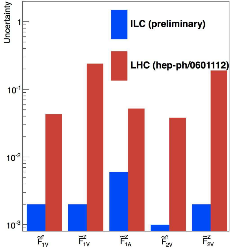
Figure 8.1: Comparison of statistical precisions on CP conserving form factors expected at the LHC [90] and at the ILC. The LHC results assume an integrated luminosity of \mathcal{L} = 300 fb^{-1} . The results of the ILC assume an integrated luminosity of \mathcal{L} = 500 fb^{-1} at \sqrt{s} = 500 GeV and a beam polarization \mathcal{P}, \mathcal{P}' = \pm 0.8, \mp 0.3 .
