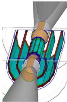
Figure 3.5: Sketch of the ILD vertex detectors.
