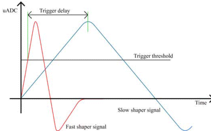
Figure 5.13: Illustration of the value of the hold and of the trigger threshold with respect to the integrated signal.
