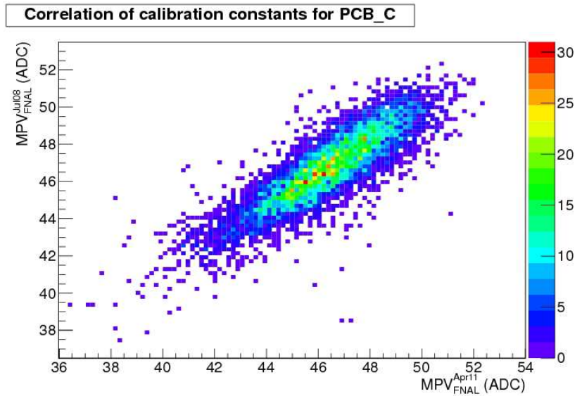
Figure A.9: Correlation of the calibration constants for the central PCBs of the two test beam periods.
