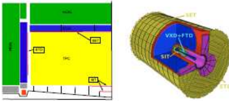
Figure 3.6: Left: a quadrant view of the ILD silicon tracking system. Right: a 3D view illustrating the position of the four components around the TPC.
