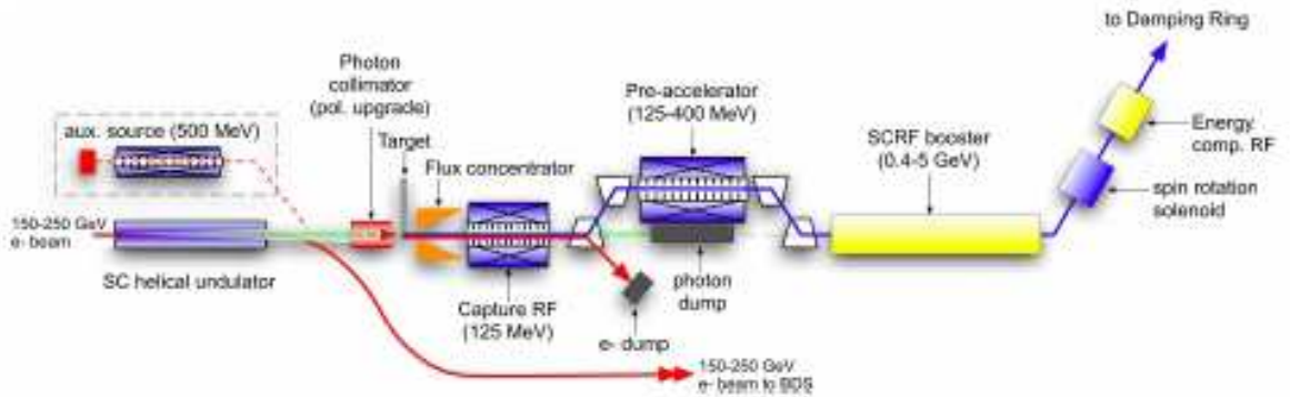
Figure 2.2: Layout of the positron source.
