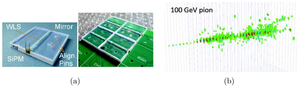
Figure 3.8: (a) AHCAL scintillator-tiles with embedded SiPMs. (b) Shower left by a 100 GeV pion in the SDHCAL prototype.
