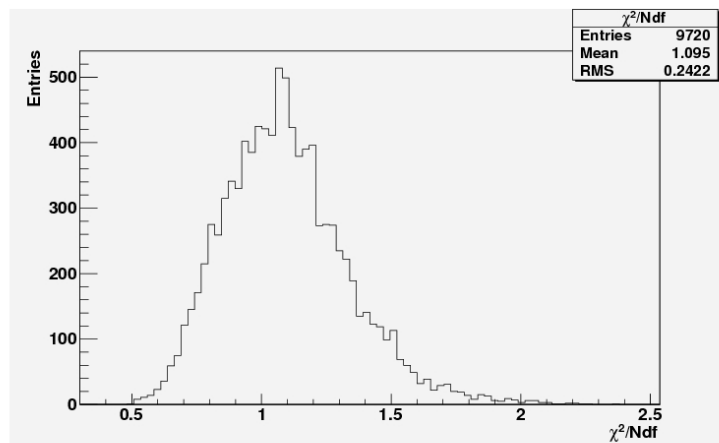
Figure A.2: Distribution of the \chi^2/Ndf for all the pads.
