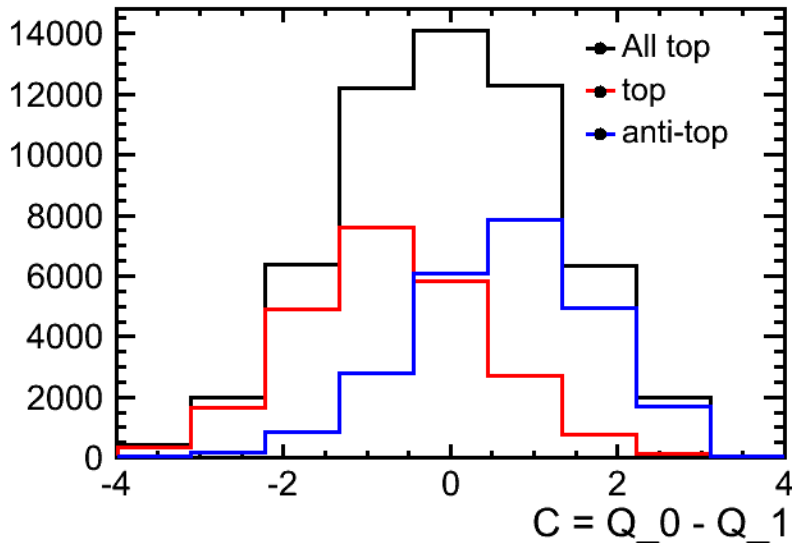
Figure 7.12: Distribution of the event charge C = Q_{b_0} - Q_{b_1} variable. The two subdistribution used the Monte Carlo truth information to know if its a top or an anti-top event.
