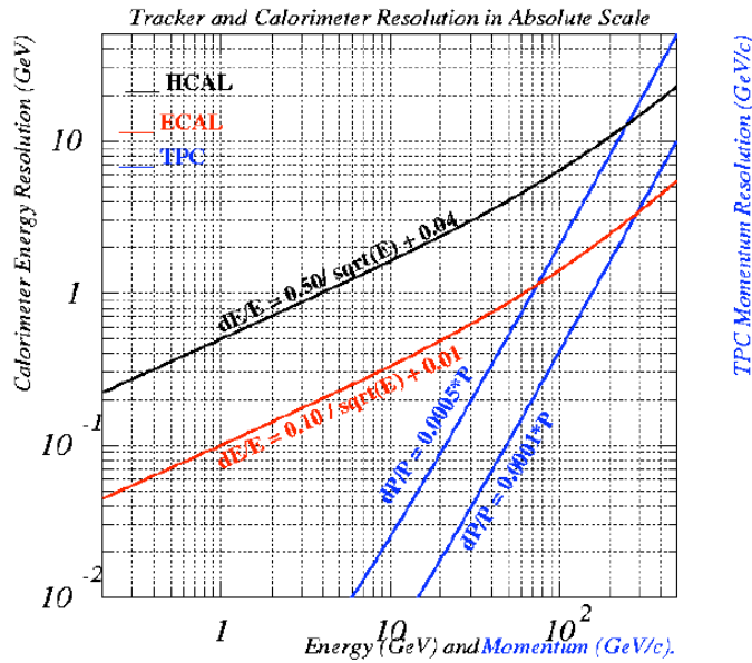
Figure 3.2: Energy and momentum resolution as provided by tracking devices (TPC) and calorimeters (ECAL, HCAL). The study presented here was performed for the TESLA detectors [33] which was similar to the ILD concepts.
