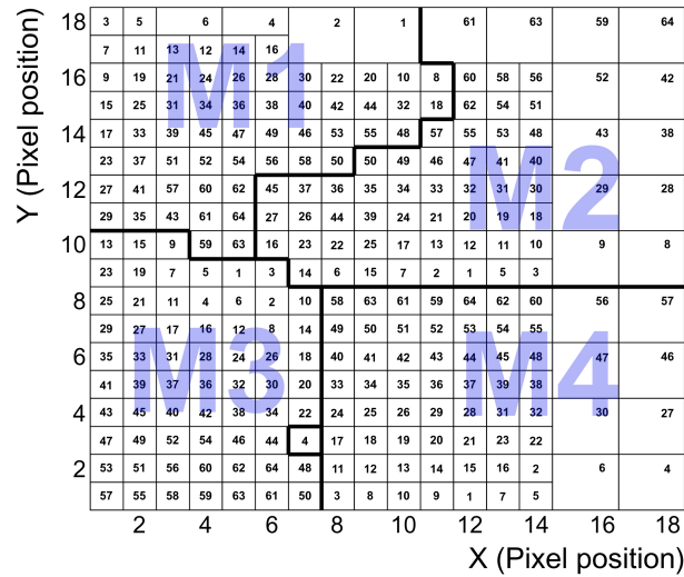
Figure 5.7: Mapping of the channels of one layer. The ASIC channels connected to sensor pixels are shown as a function of the pixel position. The broad lines represent the ASIC borders. Some ASIC channels are linked to several pixels (large boxes). The isolated channel 4 between M3 and M4 belonged to M2.
