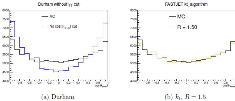
Figure 7.3: The polar angle distribution of the hadronically decaying W boson for two different jet algorithms with the \gamma\gamma \rightarrow hadrons background.
