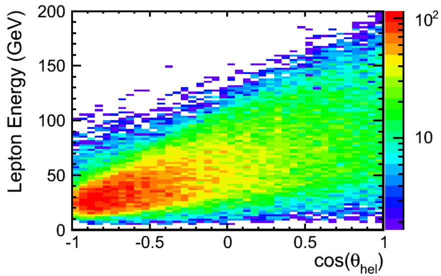
Figure 7.15: Energy distribution of the lepton with respect to its polar angle in the rest frame of the top quark.
