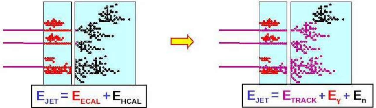
Figure 3.3: Illustration of the Particle Flow Algorithm principle.
