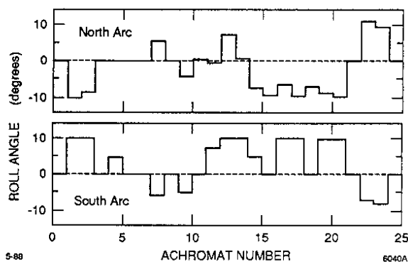
Fig. 1: Roll angle about the beam axis vs. achromat number for North and South Arcs.
