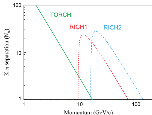
Fig. 1. Calculated performance (in sigma separation) of the different components of the LHCb PID system versus momentum, for isolated tracks [1]. The effect of angular straggling is not included.
