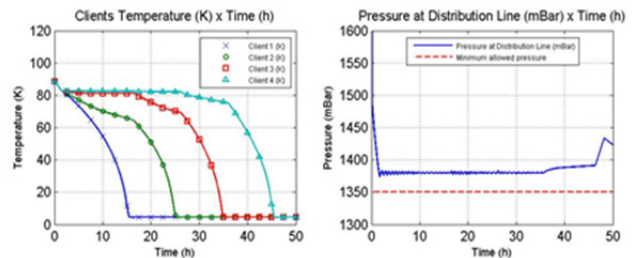
Figure 7: Cool down simulation using TBPH.
