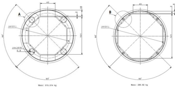
Fig.3 16mm (left) and 6mm (right) versions of the BS inside a 147 mm OD, 4 mm-thick cold bore. A radial gap of 0.2 mm is left between the BS Inermet inserts and cooling capillaries and the ID of the 1.9 K cold bore.
