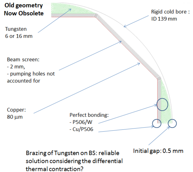
Fig.5 – Sample CASTEM calculation, showing the geometry and meshing implemented for the shielded BS.
