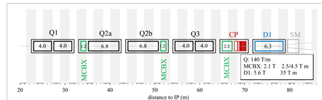
Fig.1 – Proposed HL-LHC triplet area magnet configuration
