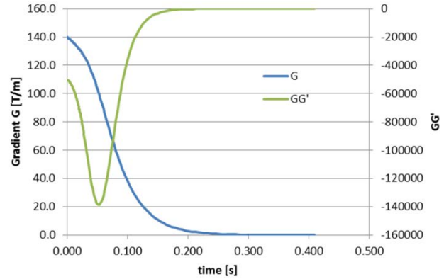
Fig.4 – Gradient G(t) (left axis), and product of it with its gradient decay G \cdot G'(t) (right axis) for an early version of the triplet magnets (140 T/m). It is G \cdot G' which ultimately determines the mechanical forces. Realistic values for the resistivity of the Inermet 180 and the co-laminated Cu-stainless steel BS have been taken into account (see R. Kersevan, in [2]).
