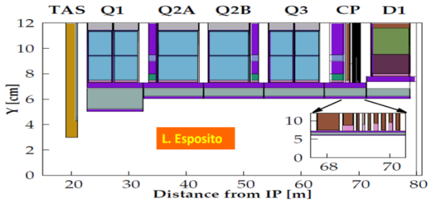
Fig.2 – Vertical cross section of the triplet area: Moving from the beam axis out radially, 2 mm-thick BS (magenta), Inermet 180 shielding (grey), 4 mm-thick cold-bore (magenta), 1.5 mm for the LHe ring (pink), cold masses (light blue).
