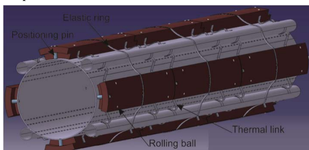
Fig.6 New concept for the BS. Cross-section to be optimized, the circular shape shown here is not representative of the final configuration.
