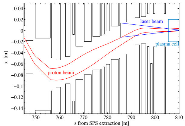
Figure 1: Horizontal chicane used to merge the laser and the proton beam. The beam envelopes and the aperture of the different elements (magnets and diagnostics) are shown.
