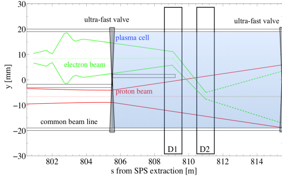
Figure 4: Common beam line for the side-injection of the electron beam into the plasma cell. The beam envelope at \pm 6 \sigma_{x,y} and \pm 3 \sigma_{x,y} is considered for protons and electrons respectively. The plasma induces a 1 mrad divergence on the proton beam. An arbitrary divergence is considered for the electrons after the merging point in the \sim 1 mm diameter plasma channel around the beam axis.
