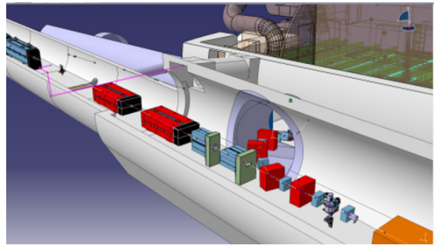
Figure 3: Layout of the merging between the proton and the electron beam lines.
