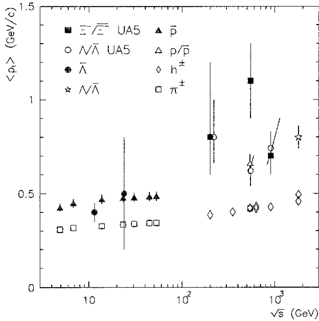
Figure 6: The average transverse momentum of \Lambda 's and \Xi^- 's plotted as a function of c.m. energy. Also shown are data from other experiments on \Lambda 's [13], protons [14,15], charged hadrons [16], and pions [14,15].
