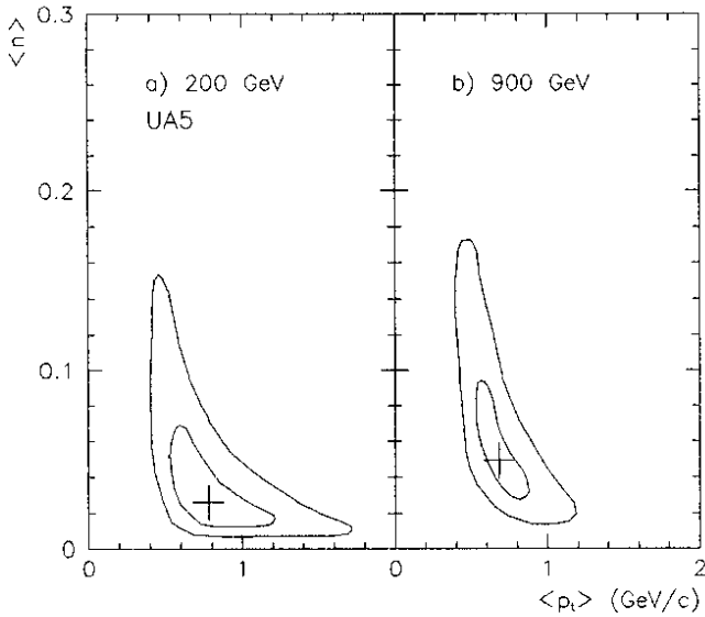
Figure 8: Contour diagrams of the \Xi^- likelihood functions at a) 200 GeV and b) 900 GeV. The contours represent 39% and 86% joint likelihood regions for \langle p_t \rangle and \langle n \rangle .
