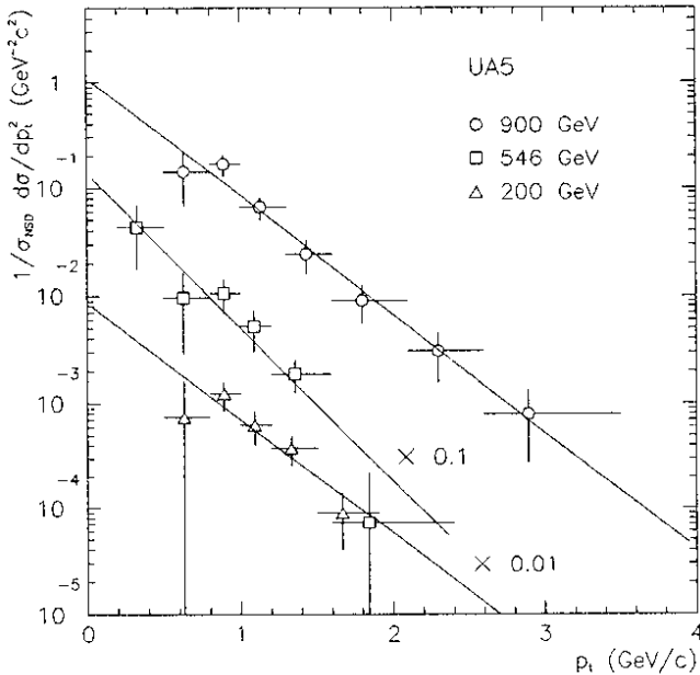
Figure 4: The corrected p_t distributions of \Lambda 's at 200, 546, and 900 GeV. The lines are exponential functions in p_t which have been fitted to the data. The 546 GeV data is from [3].
