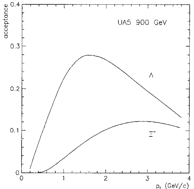
Figure 3: The \Lambda and \Xi^- acceptances at 900 GeV as a function of p_t . The acceptances do not include branching ratios. The 200 GeV acceptances are very similar.
