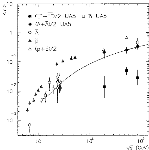
Figure 10: The yields of \Lambda 's and \Xi^- 's per inelastic event in pp(\bar{p}p) collisions as a function of c.m. energy. Data on antineutrons from this experiment [18] and data on \bar{\Lambda} 's [13,19,20] and protons [14,15] from other experiments are also shown. The 546 GeV proton yield has been estimated from a fit [9] to UA2 data [15]. Leading particles are excluded. The curve represents a fit of the function \langle n_\Lambda \rangle_{inel} = a + b \ln s + c \ln^2 s to the \Lambda data above 10 GeV. The parameter values are given in the text.
