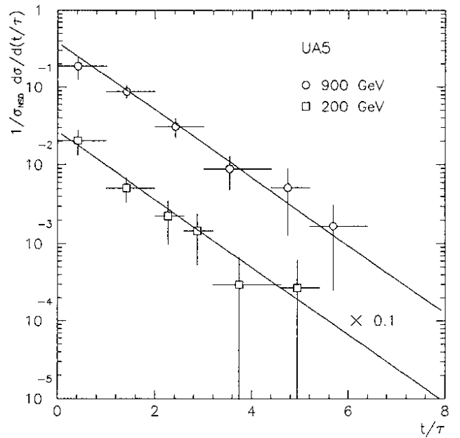
Figure 7: The corrected proper lifetime distribution of \Lambda 's at 200 and 900 GeV. The lines are exponential functions expected from the known lifetime and normalized to the \Lambda rate as determined from the p_t distributions.
