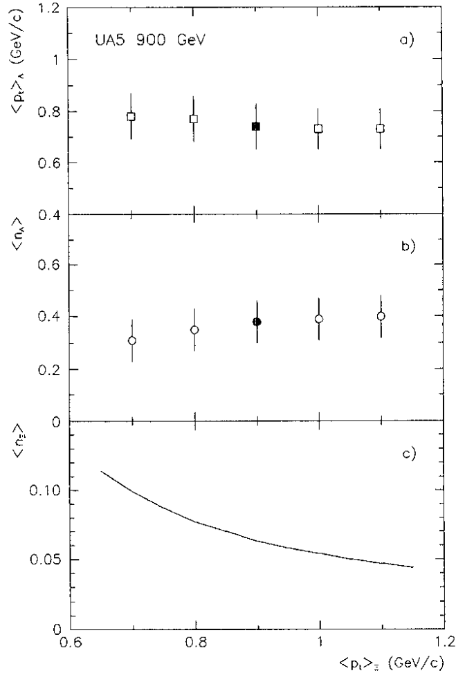
Figure 9: The dependence of a) \langle p_t \rangle_{\Lambda} , b) \langle n_{\Lambda} \rangle and c) \langle n_{\Xi^-} \rangle on the assumed value of \langle p_t \rangle_{\Xi^-} at 900 GeV. The filled markers indicate the most probable values. \langle n_{\Xi^-} \rangle and \langle p_t \rangle_{\Xi^-} have been calculated using the combined 546 and 900 GeV sample. The results at 200 GeV are similar.
