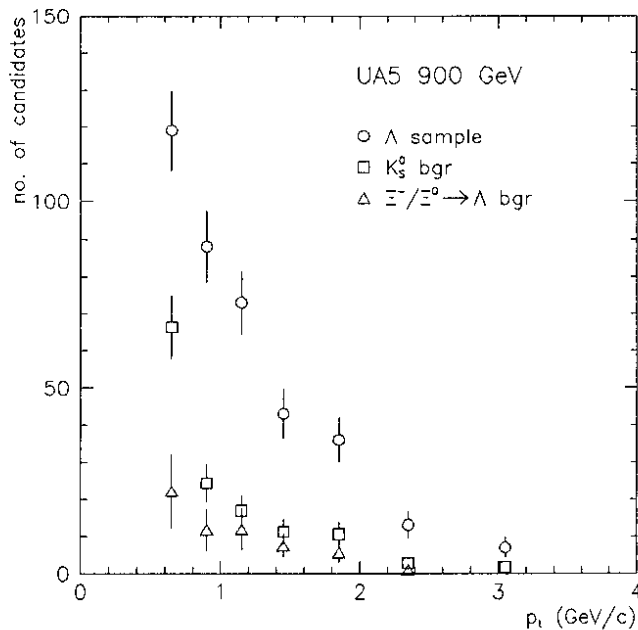
Figure 2: The observed p_t distribution of \Lambda 's at 900 GeV with the estimated background contributions from K_S^0 and \Lambda 's coming from \Xi^- and \Xi^0 decays shown. The 200 GeV distributions are similar.
