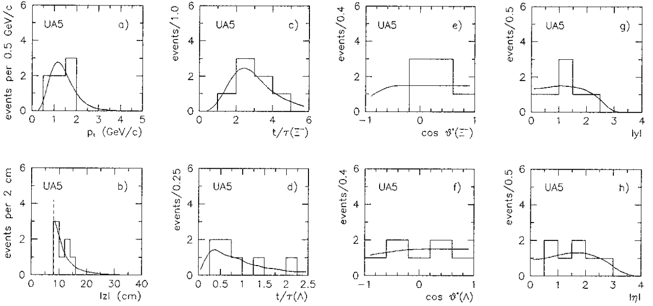
Figure 5: Observed distributions of \Xi^- 's at 900 GeV. The curves are the expected distributions calculated using MC simulation and normalized to the number of observed \Xi^- 's. The variables plotted are a) p_t , b) |z| , the z coordinate of the \Xi^- decay vertex (the dashed line indicates the position of the z cut), c) t/\tau(\Xi^-) , the proper time from the production point to the decay point of the \Xi^- , d) t/\tau(\Lambda) , the proper time from the production point to the decay point of the \Lambda from the \Xi^- decay, e) \cos\theta^*(\Xi^-) , the angle of the \Lambda in the \Xi^- rest frame, f) \cos\theta^*(\Lambda) , the angle of the proton in the \Lambda rest frame, g) |y| , and h) |\eta| .
