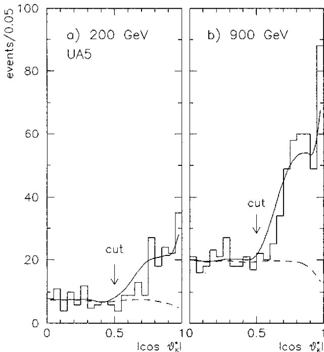
Figure 1: The |\cos\theta_K^*| distribution of V's passing the \Lambda cuts at a) 200 GeV and b) 900 GeV. The solid line is the expected distribution calculated using the measured \Lambda and \Xi^- rates and a kaon rate adjusted to give the correct number of observed candidates in the region |\cos\theta_K^*| < 0.5 . The dashed line shows the expected kaon contribution. The |\cos\theta_K^*| cut is indicated with the arrow.
