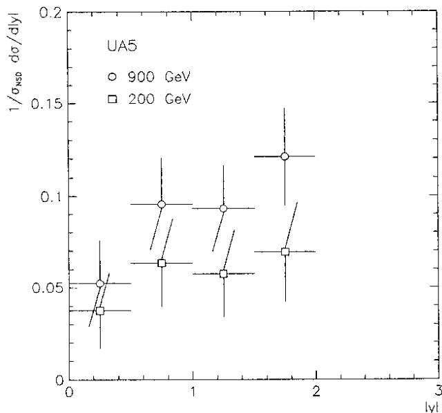
Figure 11: The rapidity distribution of \Lambda 's at 200 and 900 GeV.
