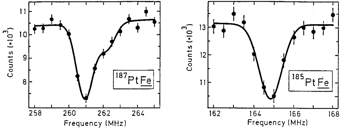
Figs. 1 and 2. NMR/ON spectra of ^{187}\text{PtFe} (712 keV) and ^{185}\text{PtFe} (460 keV) with external magnetic field of 0.1 T.
