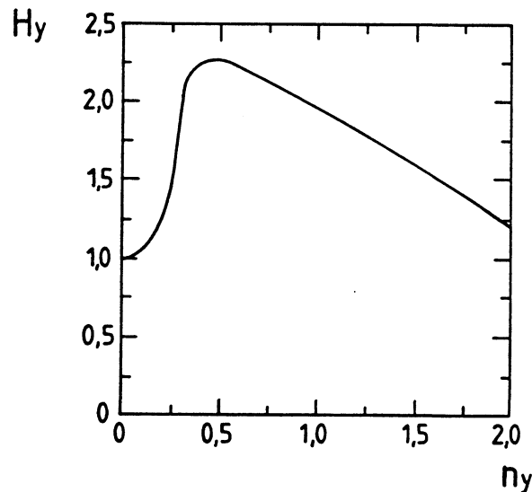
Fig. 2 Luminosity Enhancement Factor H_Y as a Function of the Beam-beam Parameter n_Y according to V.E. Balakin and N.A. Solyak (ref. 9)
