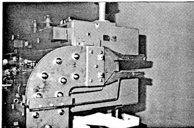
Fig. 4 - Strip-line connection for dipole magnet
