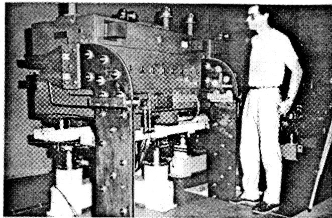
Fig. 3 - Radiation-hard pulsed dipole magnets on beam-line
