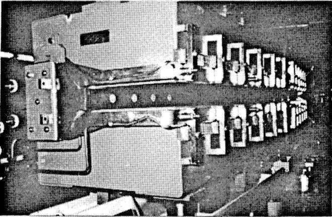
Fig. 6 - Clamping system along open side of magnet gap
