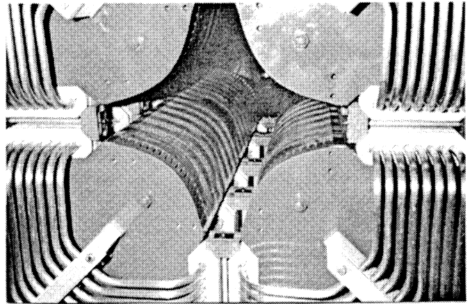
Fig. 1 - Pulsed quadrupole magnet showing coil clamps
