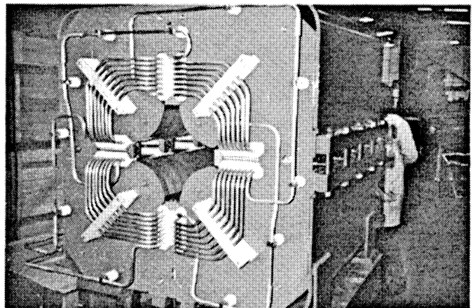
Fig. 2 - Quadrupole magnet showing coil tail mounting
