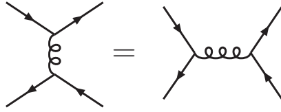
Figure 3. An additional two-term kinematic identity that can be imposed on the numerators for indistinguishable fermions in spacetime dimensions D = 3, 4, 6, 10 , or for indistinguishable complex scalars in any dimension. However, this relation is not mandatory for the color-kinematics duality. In fact, the corresponding color factors will in general not satisfy this relation.
