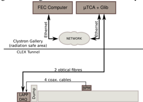
Figure 4: CTF signal processing and DAQ scheme
