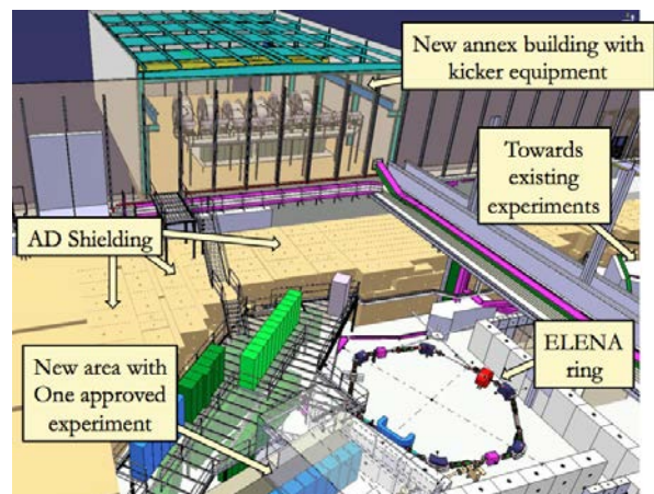
Figure 1: Sketch of the AD hall with ELENA, the new annex building and experimental areas.
