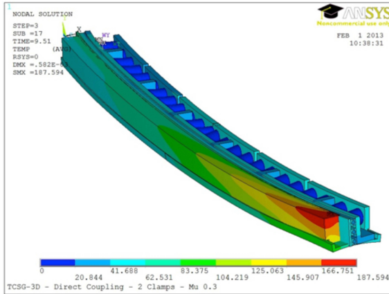
Figure 1: Collimator temperature at the end of the analysis.
