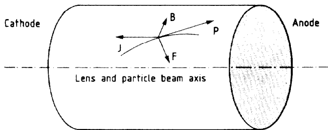
Fig. 1 Antiproton deflection inside a conducting column with current density j ; B , F , and p are the vectors of azimuthal magnetic field, force on and momentum of the particle.
