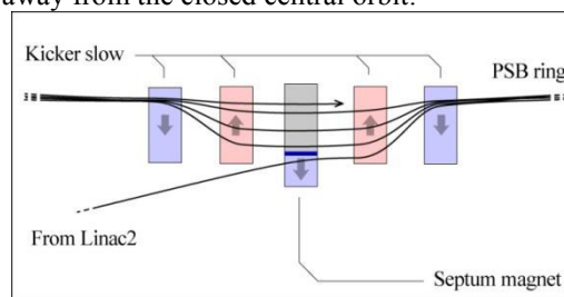
Figure 1: Multi-turn injection principle (after 4 turns).
