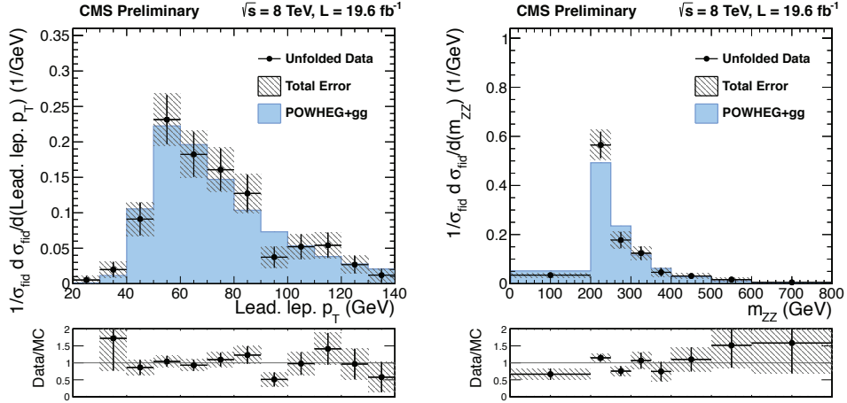
Fig. 2. – Differential cross section normalized to the fiducial cross section in the ZZ \rightarrow 2l2l' measurement at \sqrt{s} = 8 TeV, for the leading lepton p_T (left) and the invariant mass of the 4 leptons (right).
