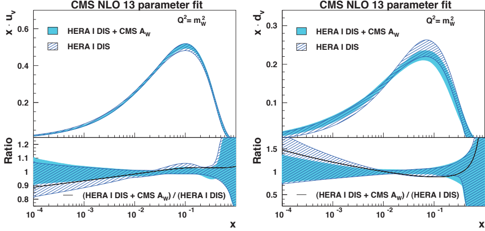
Fig. 6. – Distributions of u valence (left) and d valence (right) quarks as functions of x at the scale Q^2 = m_W^2 . The results of the 13-parameter fixed-s fit to the HERA data and muon asymmetry measurements (light shaded band), and to HERA only (dark hatched band) are compared. The total PDF uncertainties are shown.
