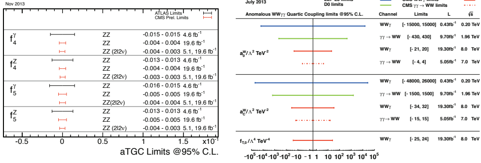
Fig. 4. – Limits on neutral aTGC ZZγ and ZZZ couplings (left) and on aQGC WWγγ dimension 6 and dimension 8 effective field theory operators couplings (right).
