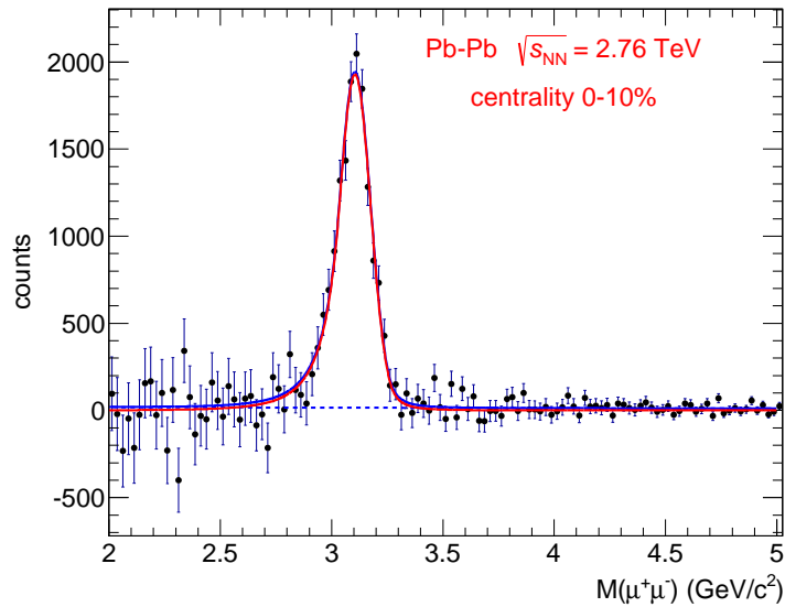
Fig. 86: Invariant-mass distribution of \mu^+\mu^- pairs in 0–10% most central Pb–Pb collisions at \sqrt{s_{\text{NN}}} = 2.76 \text{ TeV} with the J/\psi peak fitted by an extended Crystal Ball function. The combinatorial background was determined by the event mixing method and subtracted.
