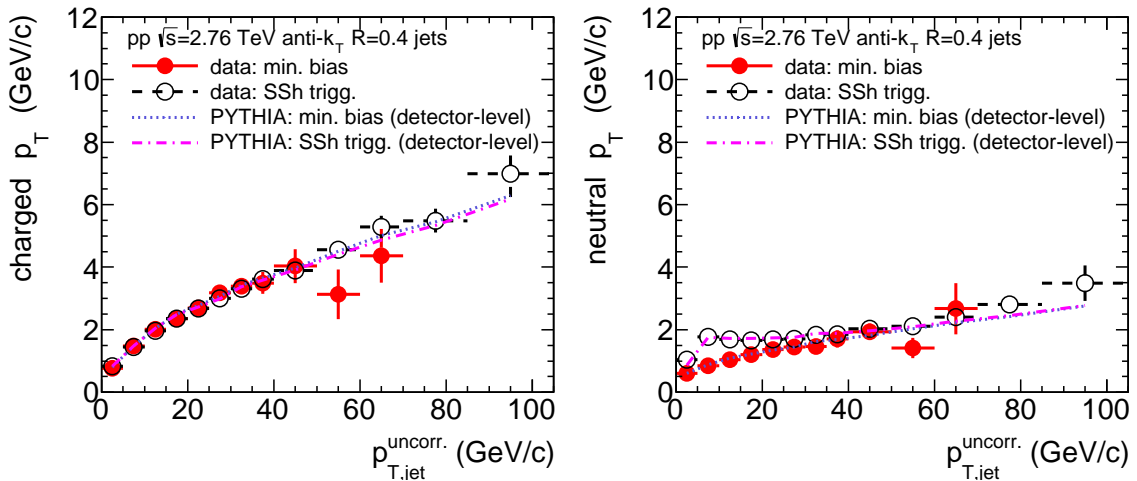
Fig. 76: Mean transverse momentum, \langle p_{\text{T}} \rangle , of constituents measured in reconstructed jets in 2.76 TeV pp collisions (anti- k_{\text{T}} , R = 0.4 ) vs. jet p_{\text{T}} . Left: charged tracks; Right: neutral clusters. Data are shown for MB and SSh triggers, and are compared to detector-level simulations.
