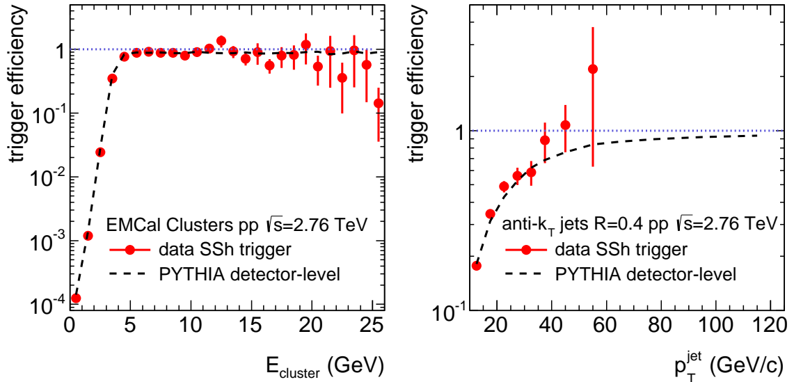
Fig. 73: SSh trigger efficiency in pp collisions at \sqrt{s} = 2.76 TeV. Efficiency for single EM clusters (left panel) and reconstructed jets (anti-kT, R = 0.4 , right panel) for data (red points) is well reproduced in simulation (black dashed line). See text for details.
