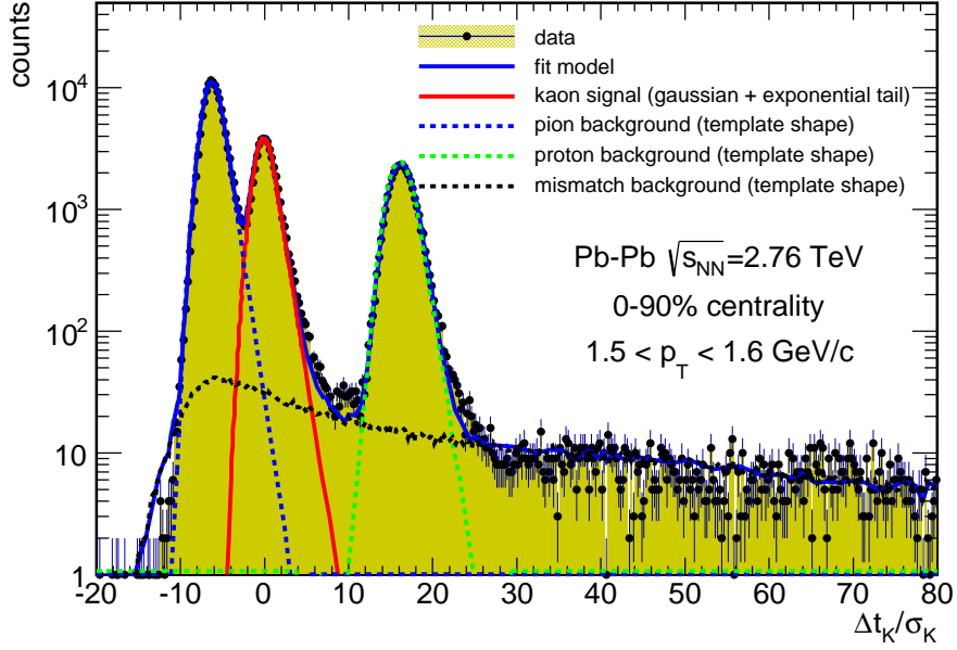
Fig. 42: TOF measured in Pb–Pb collisions at \sqrt{s_{NN}} = 2.76 TeV. The expected time of flight for kaons is subtracted and the result is divided by the expected resolution.
