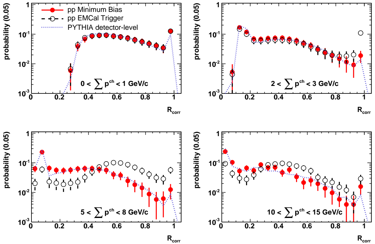
Fig. 75: Probability distribution of R_{\text{corr}} (Eq. (18)) for various intervals of \Sigma_p , measured in MB and EMCal-triggered pp collisions, compared to detector-level simulations based on PYTHIA.
