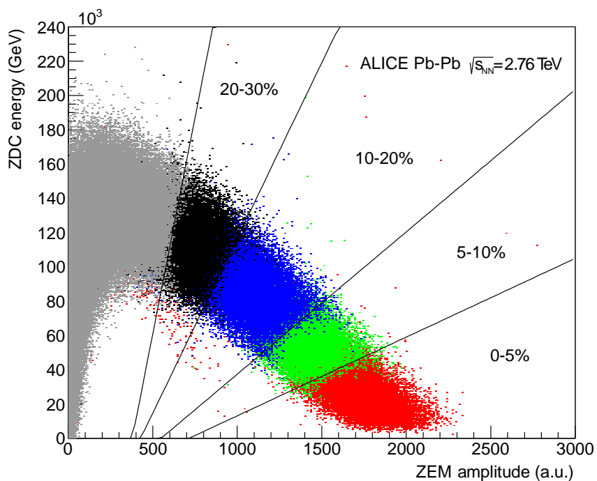
Fig. 12: Correlation between the total energy deposited in the zero-degree calorimeters and the ZEM amplitude. The centrality bins defined based on this distribution (lines) are compared to the centrality from V0 (colored dots).
