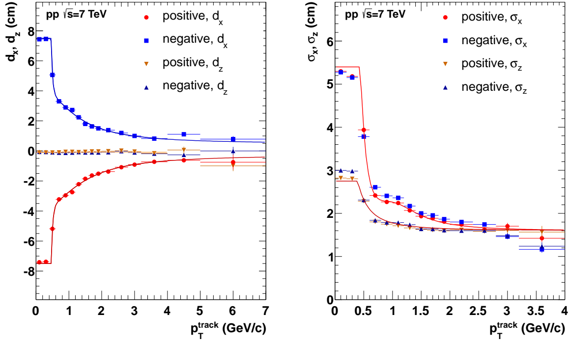
Fig. 63: Mean track matching distance (left) and RMS of the track matching distance distribution (right) for PHOS. The lines are fits to phenomenological parameterizations.
