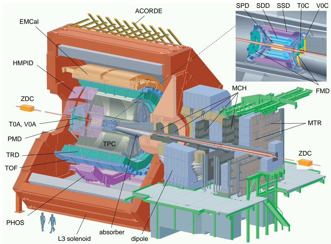
Fig. 1: The ALICE experiment at the CERN LHC. The central-barrel detectors (ITS, TPC, TRD, TOF, PHOS, EMCal, and HMPID) are embedded in a solenoid with magnetic field B = 0.5 \text{ T} and address particle production at midrapidity. The cosmic-ray trigger detector ACORDE is positioned on top of the magnet. Forward detectors (PMD, FMD, V0, T0, and ZDC) are used for triggering, event characterization, and multiplicity studies. The MUON spectrometer covers -4.0 < \eta < -2.5 , \eta = -\ln \tan(\theta/2) .
