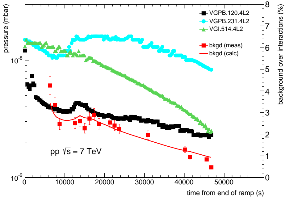
Fig. 3: Beam pipe pressure and background rate in fill 2181. The expected background rate has been estimated using the linear parameterization shown in Fig. 2. VGPB.120.4L2, VGPB.231.4L2, and VGI.514.4L2 are the pressure gauges located in front of the Inner triplet (at 69.7 m from IP2), on the TDI beam stopper (at 80 m from IP2), and on the large recombination chamber (at 109 m from IP2), respectively.
