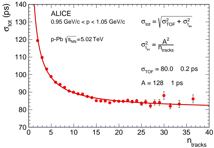
Fig. 41: Time resolution of pion tracks with 0.95 < p < 1.05 \text{ GeV}/c as a function of the number of tracks used to define the start time of the collision t_{ev} [64]. The data are from p–Pb collisions.
