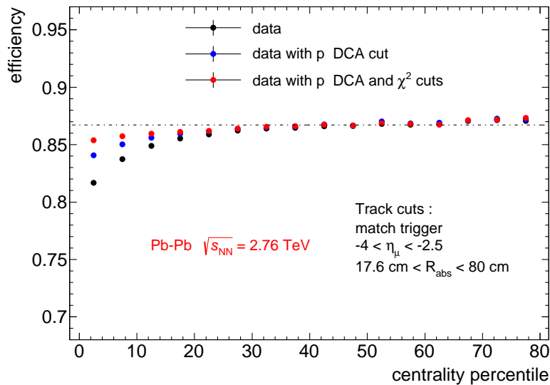
Fig. 82: Measured muon track reconstruction efficiency in Pb–Pb collisions as a function of the collision centrality.
