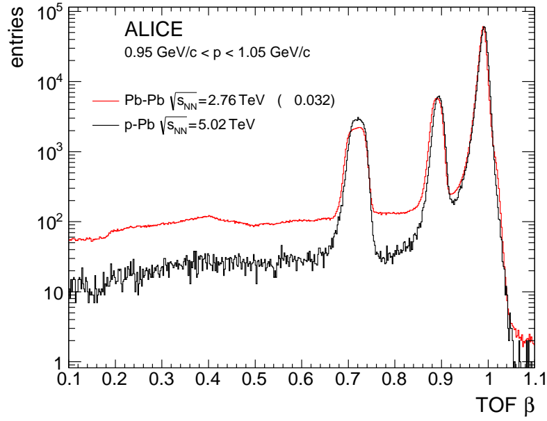
Fig. 40: TOF \beta distribution for tracks with momentum 0.95 \text{ GeV}/c < p < 1.05 \text{ GeV}/c . The Pb–Pb histogram is normalized to the p–Pb one at the pion peak ( \beta = 0.99 ) While the resolution (width of the mass peaks) is the same, the background of mismatched tracks increases in the high-multiplicity environment of Pb–Pb collisions. Both samples are minimum bias.
