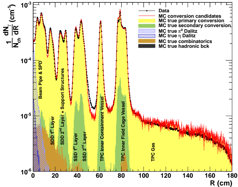
Fig. 67: Radial distribution of the reconstructed photon conversion points for |\eta| < 0.9 (black) compared to MC simulations performed with PHOJET (red). Distributions for true converted photons are shown in yellow. Physics contamination from true \pi^0 and \eta Dalitz decays, where the primary e^+e^- are reconstructed as photon conversions, are shown as dashed blue histograms. Random combinatorics and true hadronic background are also shown.
