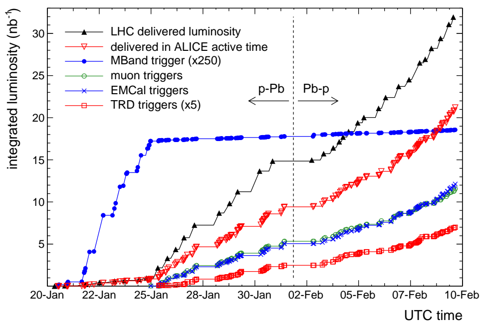
Fig. 10: Integrated luminosity in the 2013 p–Pb run.
