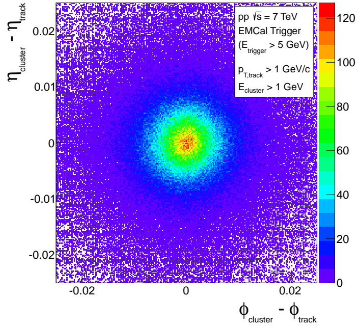
Fig. 52: Distribution of the residuals for the EMCal clusters to track matching in pseudorapidity ( \eta_{\text{cluster}} - \eta_{\text{track}} ) vs. azimuth ( \phi_{\text{cluster}} - \phi_{\text{track}} ) in pp collisions at \sqrt{s} = 7 TeV triggered by EMCal. Only clusters with an energy E_{\text{cluster}} > 1 GeV and tracks with a transverse momentum p_{T,\text{track}} > 1 GeV/c are used.
