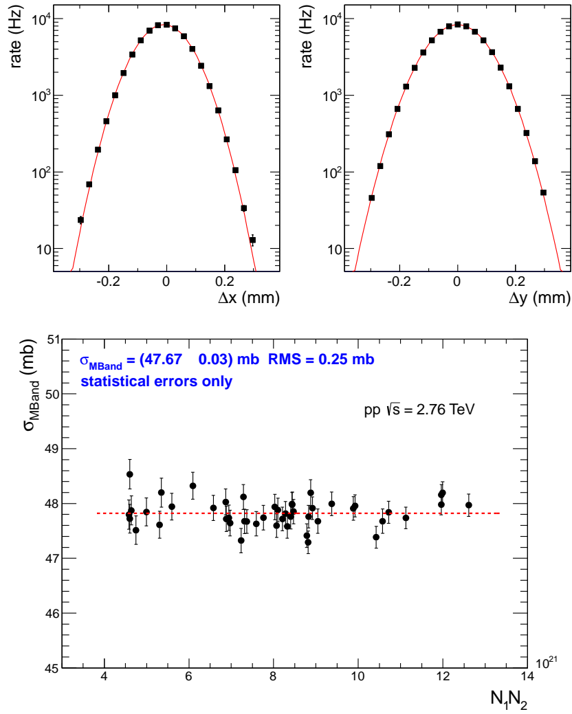
Fig. 8: Top: MBand trigger rate vs. beam separation in x and y obtained during the May 2010 van der Meer scan. Double Gaussian fits to the data are shown as lines. Bottom: Measured MBand cross section for 48 colliding bunch pairs in the March 2011 scan, as a function of the product of colliding bunch intensities N_1 N_2 .
