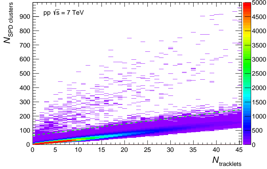
Fig. 6: Correlation between reconstructed SPD clusters and tracklets. Two bands corresponding to the collisions and MIB are visible. The dashed cyan line represents the cut used in the offline selection: events lying in the region above the line are tagged as BG and rejected.
