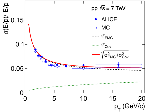
Fig. 54: Relative resolution of E/p vs. transverse momentum p_T for electrons in experimental data (full dots) and from a fully reconstructed MC (open circles) in pp collisions at \sqrt{s} = 7 TeV. The EMCal energy resolution deduced from the width of the \pi^0 and \eta invariant mass peaks (black dotted line), added in quadrature to the TPC p_T resolution (green dash-dotted line), describes the measurement reasonably well (red solid line).
