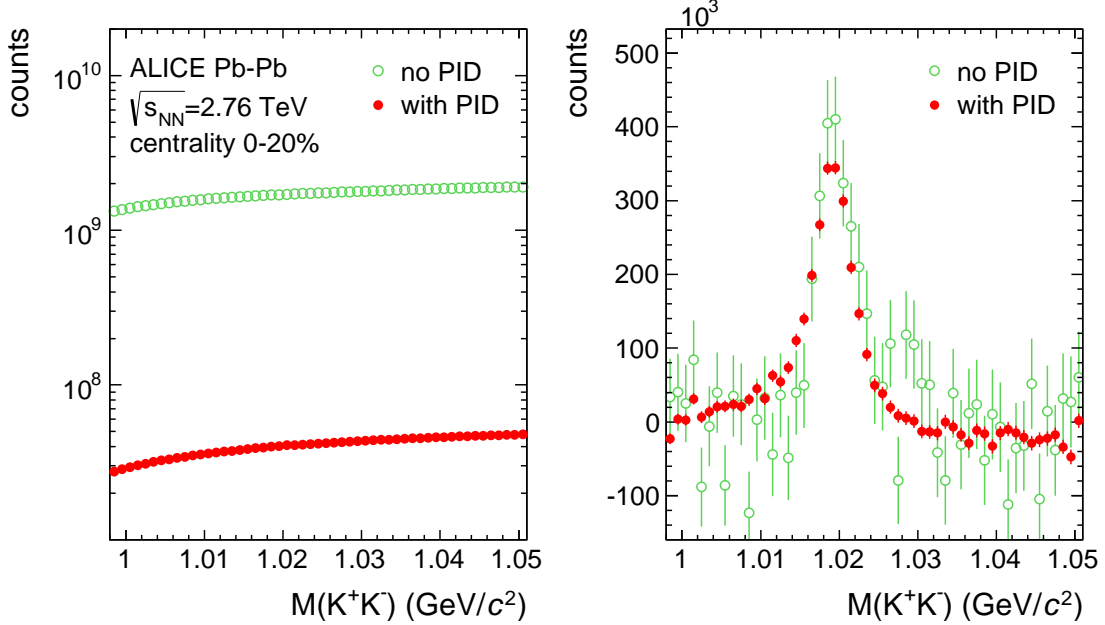
Fig. 49: Invariant mass distribution of K^+K^- candidate pairs for reconstruction of the \phi \rightarrow KK decay, with and without particle identification, before (left panel) and after (right panel) background subtraction.
