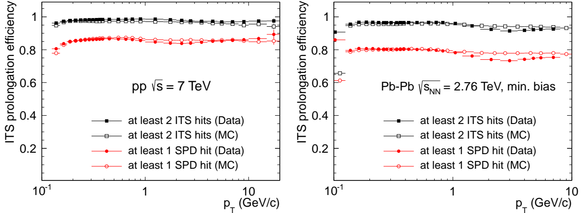
Fig. 20: ITS–TPC matching efficiency vs. p_T for data and Monte Carlo for pp (left) and Pb–Pb (right) collisions.
