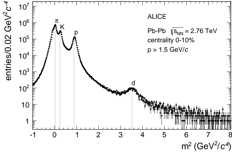
Fig. 45: Squared particle masses calculated from the momentum and velocity determined with ITS-TPC and HMPID, respectively, in central Pb-Pb collisions at \sqrt{s_{NN}} = 2.76 TeV. The velocity is calculated from the Cherenkov angle measured in the HMPID. Dotted lines indicate the PDG mass values. The pion tail on the left-hand side is suppressed by an upper cut on the Cherenkov angle. The deuteron peak is clearly visible.
