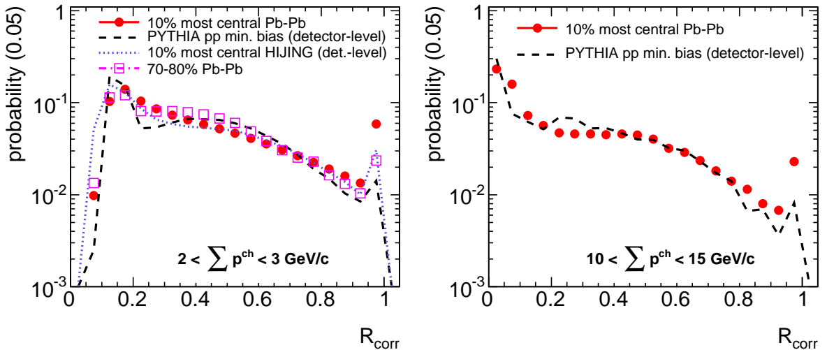
Fig. 80: Probability distribution of R_{\text{corr}} (Eq. (18)) in two different intervals of \Sigma_p , measured in central (0–10%) and peripheral (70%–80%, left panel only) Pb–Pb collisions. Also shown are detector-level simulations for MB pp collisions based on PYTHIA (same distributions as Fig. 75), and for central Pb–Pb collisions based on HIJING (left panel only).
