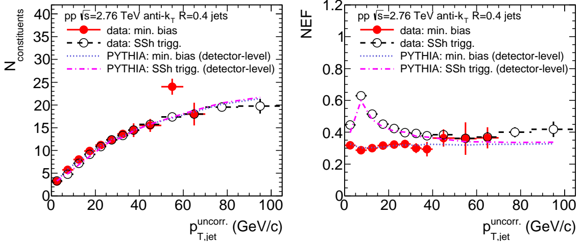
Fig. 77: Mean total number of constituents (left) and mean neutral energy fraction (right) measured in reconstructed jets in 2.76 TeV pp collisions (anti- k_T , R = 0.4 ), vs. jet p_T . Data are shown for MB and SSh triggers, and are compared to detector-level simulations.
