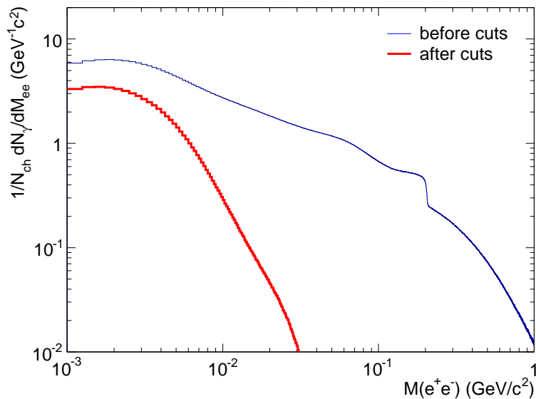
Fig. 65: Invariant mass distribution of all reconstructed secondaries (blue) and of the selected photon candidates (red) after all cuts were applied.
