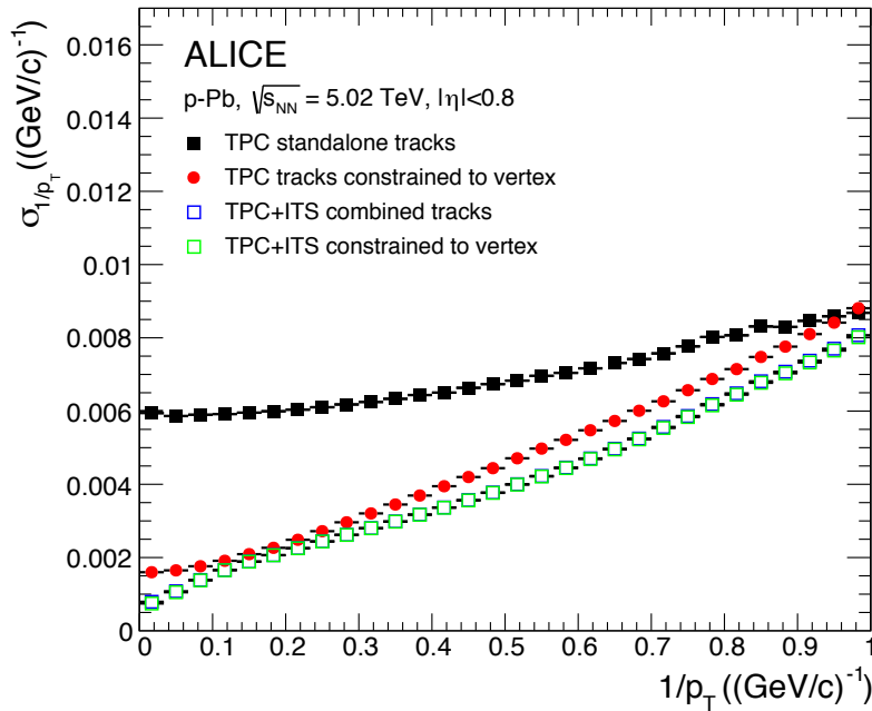
Fig. 23: The p_T resolution for standalone TPC and ITS–TPC matched tracks with and without constraint to the vertex. The vertex constrain significantly improves the resolution of TPC standalone tracks. For ITS–TPC tracks, it has no effect (green and blue squares overlap).
