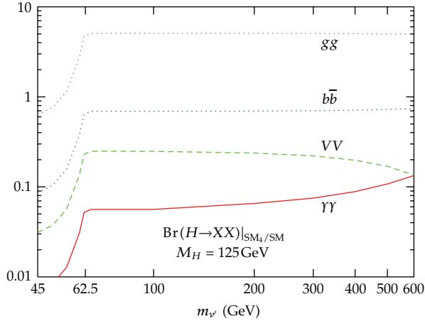
FIGURE 7: Higgs branching ratios in dependence of the mass of the fourth neutrino for a Higgs mass of 125 GeV. Below m'_\nu = 62.5 GeV the new invisible decay channel H \rightarrow \nu_4 \nu_4 opens and all other branching ratios will be strongly suppressed. This plot was, however, created with an approximate NLO expression for H \rightarrow \gamma\gamma . The full expression will give a further suppression of the two-photon channel by a factor of about six. Figure taken from [17].
