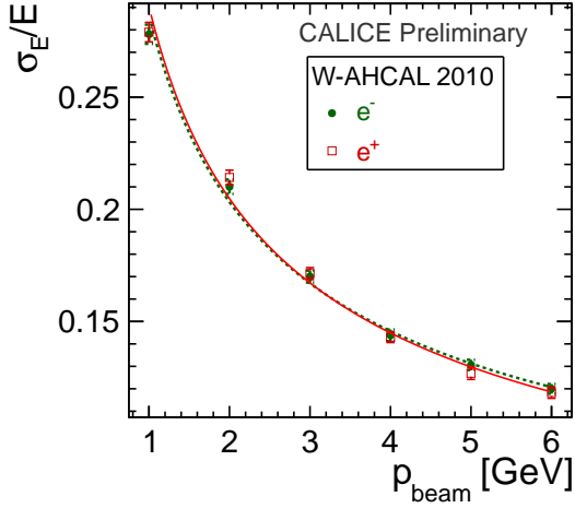
Figure 17: Energy resolution for the 2010 e^+/e^- W-AHCAL data. The error bars are given by the quadratic sum of the statistical and systematic errors.
