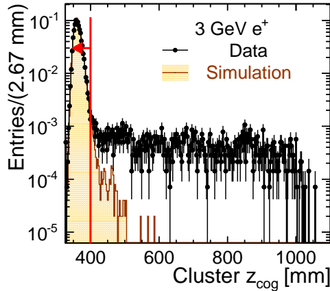
Figure 10: Distribution of the z_{\text{cog}} of clusters identified in 3 GeV e^+ events.
