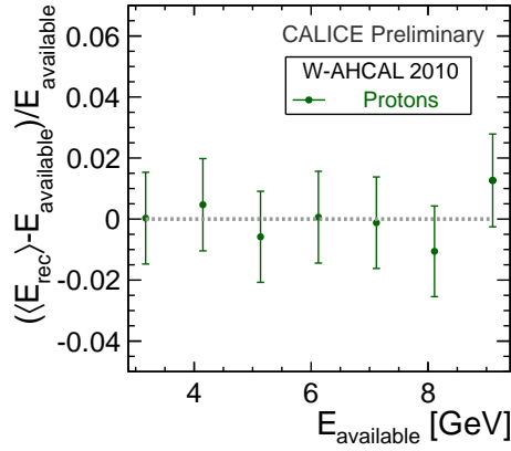
Figure 44: Deviations from linearity for the W-AHCAL 2010 proton data.
