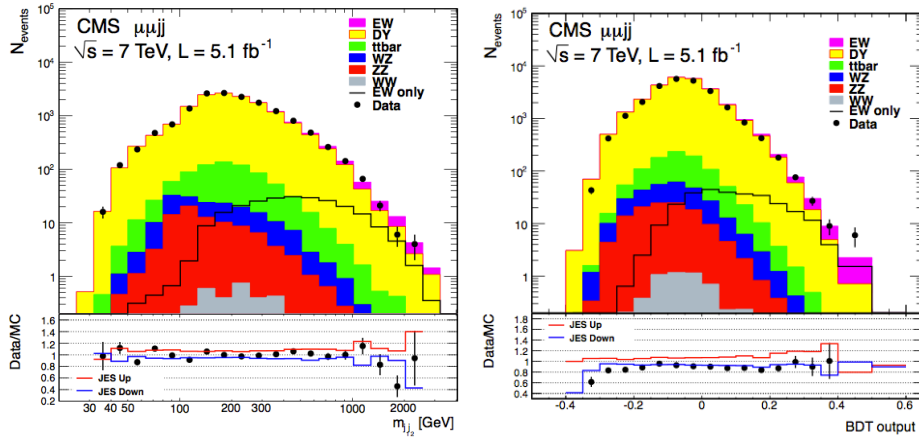
Figure 2: Dijet invariant mass left and BDT output ( right ) for the dimuon channel after selecting the Z candidate and the tag jets. The expected contributions from the signal and background processes are evaluated from simulation. The solid line with the label “EWK only” shows the distribution for the signal alone. The bottom panels show the ratio of data over the expected contribution of the signal plus background. The region between the two lines, with the labels JES Up and JES Down, shows the 1\sigma uncertainty of the simulation prediction due to the jet energy scale uncertainty. The data points are shown with the statistical uncertainties.
