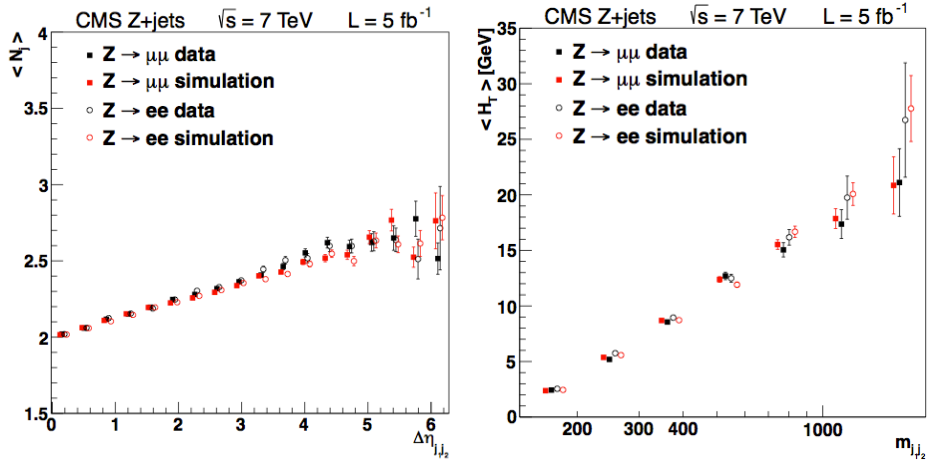
Figure 3: Left: average number of jets with p_T > 40 GeV as a function of the \Delta\eta_{j_1j_2} separation. Right: average H_T of the three leading soft track jets in the pseudo-rapidity interval between the tagging jets for p_T^{j_1,j_2} > 65, 40 GeV as a function of the dijet invariant mass. The data points and the points from simulation are shown with the statistical uncertainties.
