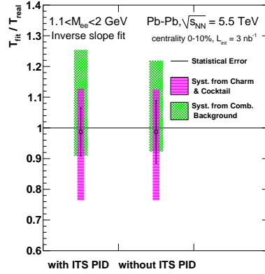
Figure 8.27: Expected relative uncertainty on the extraction of the T parameter from a fit to the invariant mass excess spectrum in 1.1 < M_{ee} < 2 GeV/ c^2 (see text). The results are shown for different scenarios, with tight d_0 cuts, and for 0–10% event centrality. Error bars show the statistical uncertainties. The green boxes show the systematic uncertainties from the combinatorial background subtraction, the magenta boxes indicate systematic uncertainties related to the subtraction of the cocktail and charm contribution.
