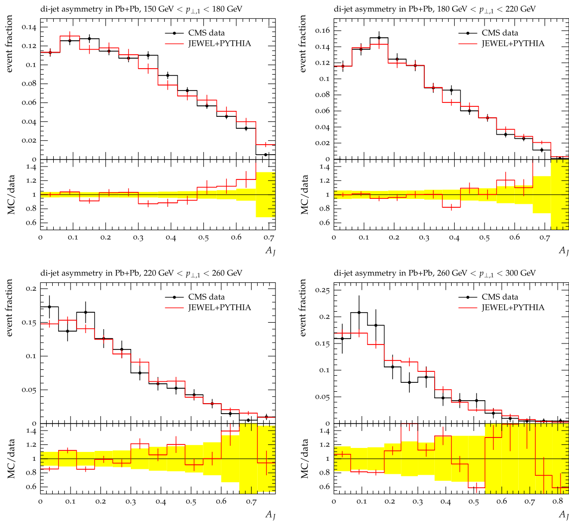
Fig. 10 Di-jet asymmetry A_J = (p_{\perp,1}p_{\perp,2})/(p_{\perp,1} + p_{\perp,2}) in Pb+Pb collisions (0–20% centrality) for different transverse momenta of the leading jet. The sub-leading jet is required to have p_{\perp,2} > 30 GeV and
