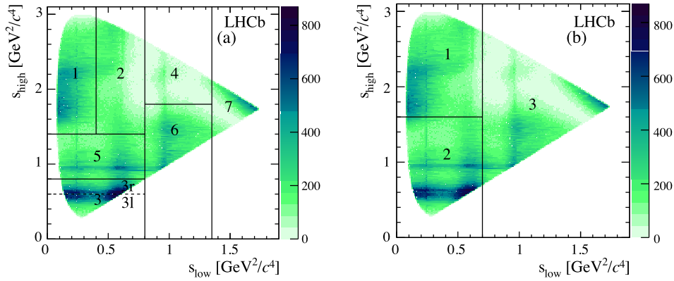
Fig. 11. Dalitz plot for D^+ \rightarrow \pi^- \pi^+ \pi^+ candidates divided into (a) seven regions R1–R7 and (b) three regions P1–P3.
