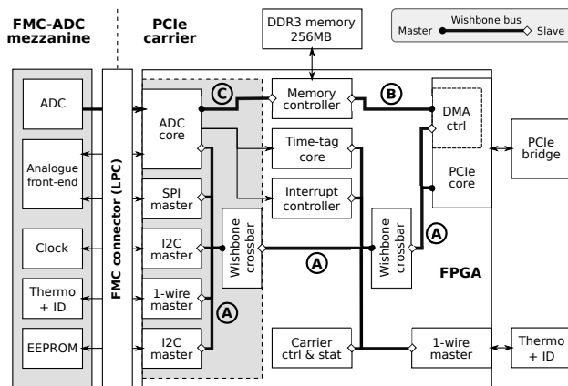
Figure 2: FMC-ADC gateway architecture.
