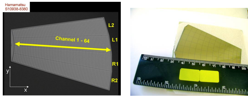
Figure I-2.5 Prototypes sensors for LumiCal (left) and BeamCal (right).
