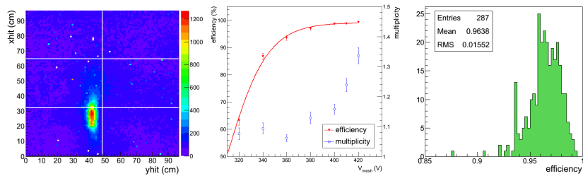
Figure II-4.19 Muon beam profile using internal trigger mode (left) efficiency and pad multiplicity.
