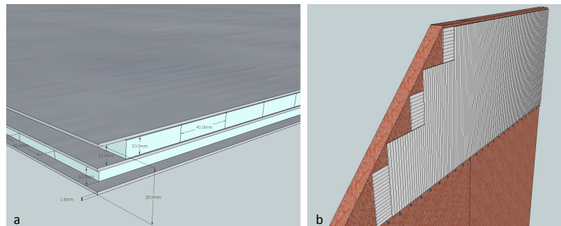
Figure II-5.4 (left) Each gap in the barrel flux return is filled by two orthogonal planes of scintillating strips glued to three aluminium sheets to form a rigid rectangular sandwich. (right) The endcap modules are \approx 1.8 m high to slide between the spacers separating the endcap steel layers.
