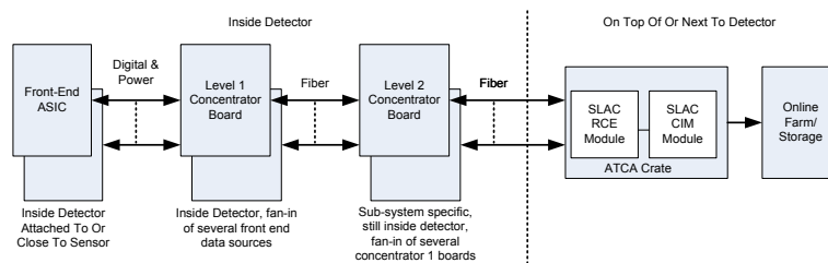
Figure II-9.1 Simplified block-diagram of the SiD detector control and readout chain using the ATCA RCE and CIM modules (defined later in this chapter).
