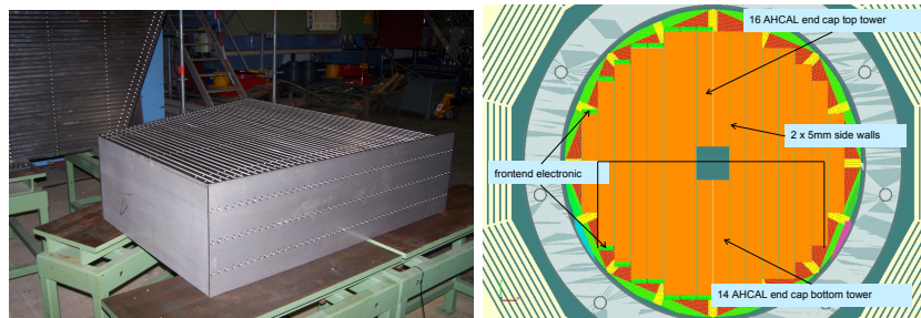
Figure III-3.13 Left: the mechanical prototype for the first version of the barrel structure. Right: mechanical design of the HCAL endcap.
