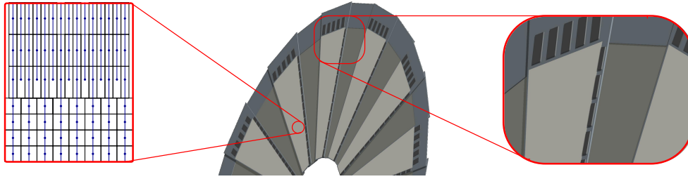
Figure III-2.10. A half-disk for the FTD in the DEPFET petal concept. The rightmost zoom image shows a detail of the end-of-petal area that houses the read-out electronics and the balcony with the steering chips. The leftmost image shows the region at R = 8 cm where both the column width and the R -dimension of the pixels changes.
