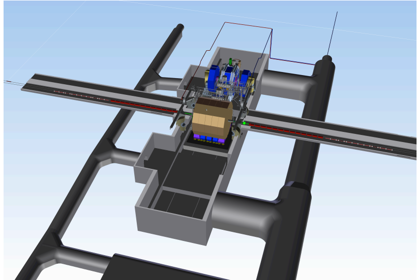
Figure I-2.13 The experimental hall for mountainous ILC sites.
