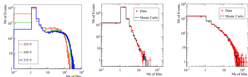
Figure II-4.20 Hit distribution from 150 GeV pions traversing a 20 cm thick iron block at various mesh voltages (left). Hit distributions from 100 GeV muons (centre) and pions (right) at layer 48 of the CALICE Fe/GRPC SDHCAL.
