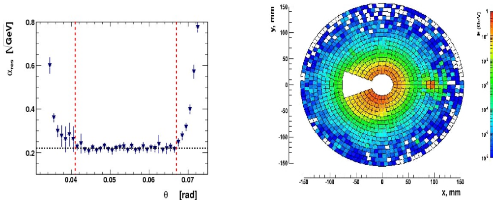
Figure III-3.25. Left: The energy resolution, \alpha_{\text{res}} , for electrons as a function of the polar angle, covering the range of LumiCal. Right: The distribution of the energy deposited by beamstrahlung pairs after one bunch crossing in the sensors of BeamCal at a depth of 5 radiation lengths. Superimposed is the deposition of a single high energy electron, seen as red spot on the right side.
