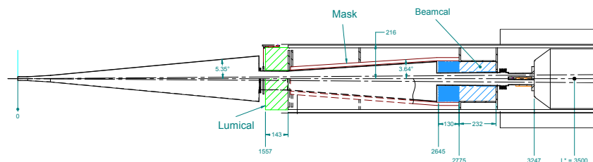
Figure II-8.1 The SiD forward region.
