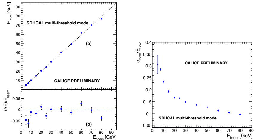
Figure III-3.21 Reconstructed energy linearity (left) and energy resolution (right) for Pions using a weighted sum of the three-threshold number of hits and with no data correction, for the SDHCAL prototype [320].
