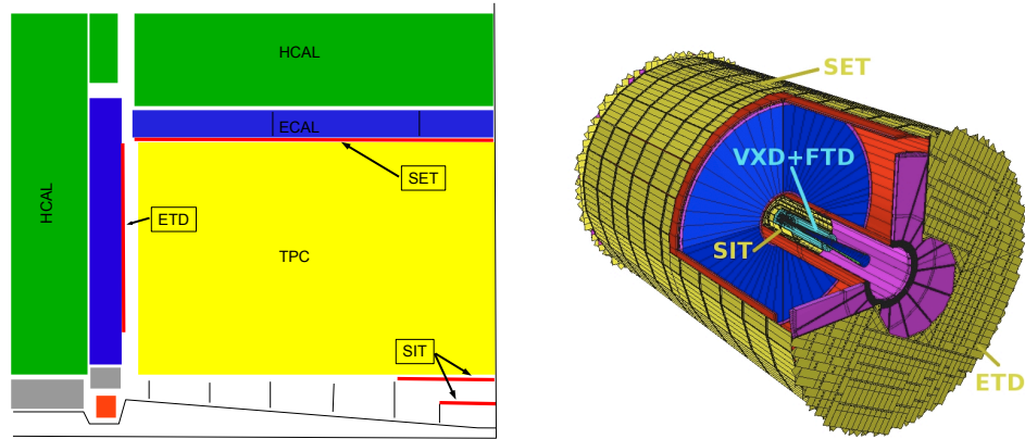
Figure III-2.8. Left: a quadrant view of the ILD silicon envelope system made of four components, SIT, SET, FTD, and ETD as included in MOKKA full simulation. Right: a 3D detailed GEANT 4 simulation description of the silicon system as sketched in the quadrant view on the left.
