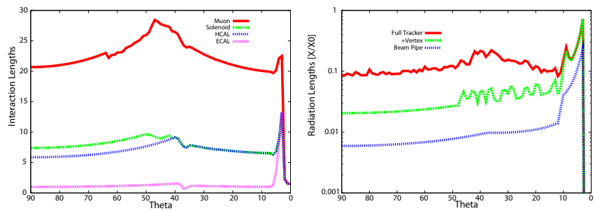
Figure II-10.4 The nuclear interaction lengths of SIDLOI3 (left) and the radiation lengths of SIDLOI3 tracking system (right) as a function of the polar angle \theta .
