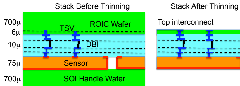
Figure II-2.3 Wafer stack structure before and after thinning and singulation.
