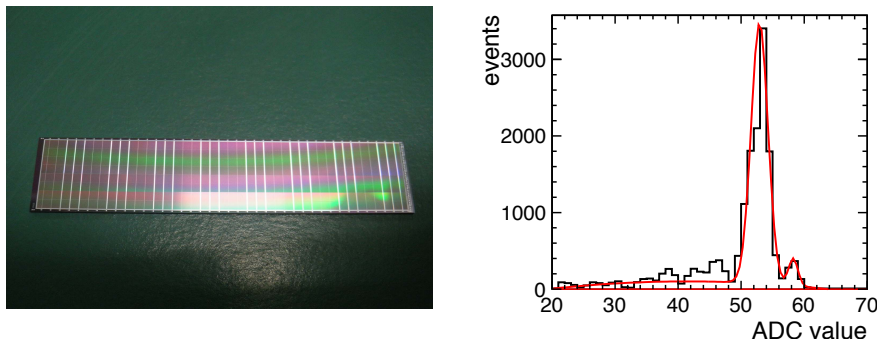
Figure III-2.3 Full size FPCCD prototype (left) and response to a ^{55}\text{Fe} source (right).
