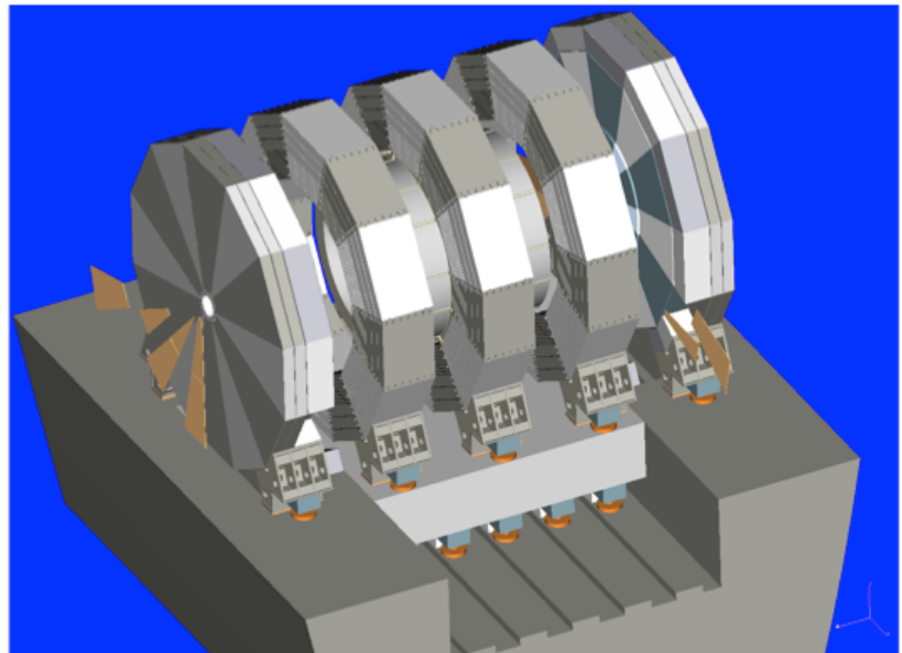
Figure III-5.1 The mechanical design of ILD.
