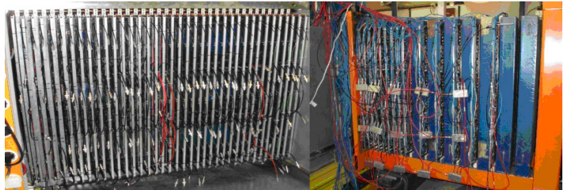
Figure II-4.11 Left: the DHCAL main stack (before cabling), right: the TCMT.
