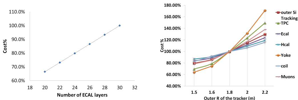
Figure III-7.3. Left: Dependence of the SiECAL cost on the number of sensitive layers. (right) Scaling of the cost of the ILD detector if the transverse size is changed, split into relative cost changes for the different sub-detectors.
