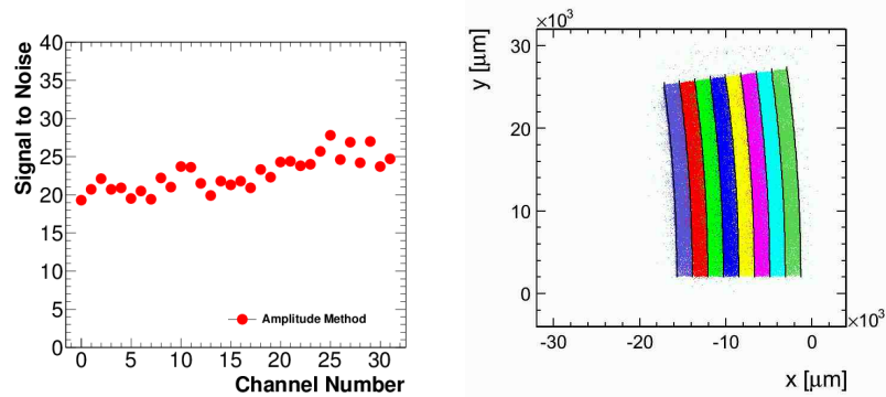
Figure III-3.29 Left: The signal-to-noise ratio of all read-out channels before calibration. Right: Distribution of the predicted impact points on pads with a colour coded signal.
