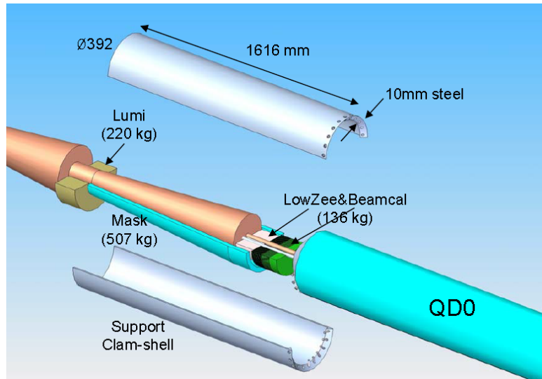
Figure II-7.5 Detail of the LumiCal, mask and BeamCal which must be supported by the QD0 support tube and alignment system.
