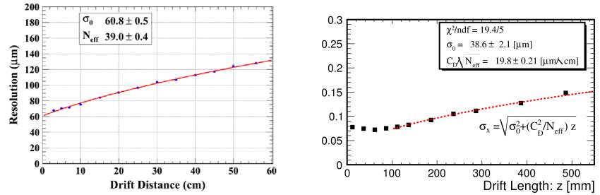
Figure III-2.16 Preliminary results from the large prototype running at 1 Tesla magnetic field, for (left) a micromegas readout [258] and (right) a GEM based readout [276]
