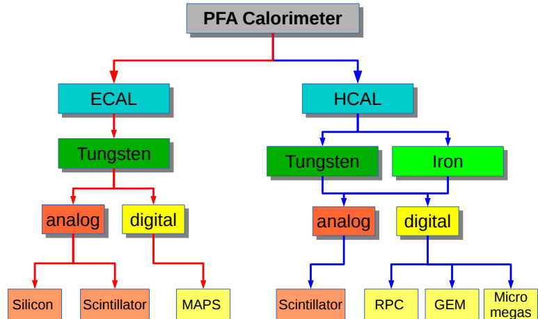
Figure I-2.1 Tree of electromagnetic calorimeter technologies -ECAL- (left) and hadron calorimeter technologies -HCAL- (right).
