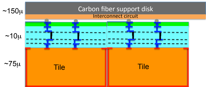
Figure II-2.4 Tiled structure used for the disk layers utilising a carbon-fibre backing disk.
