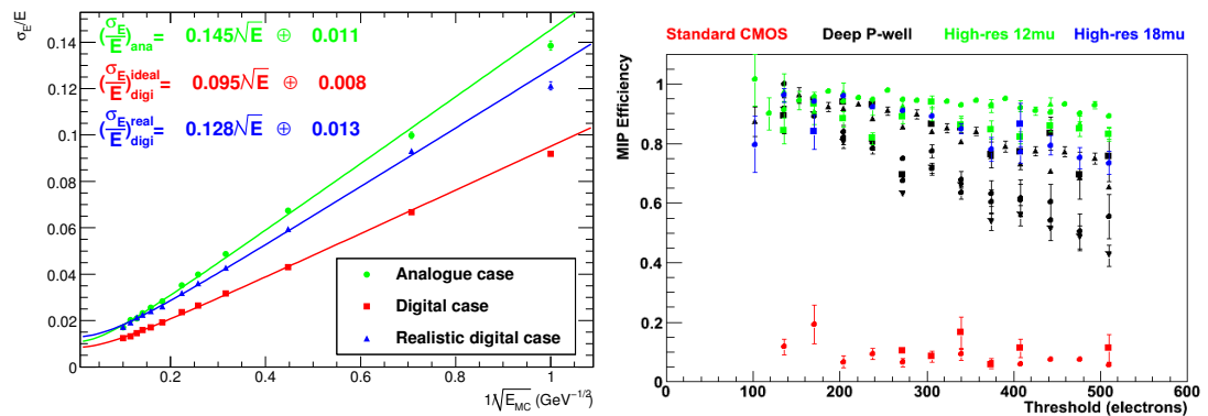
Figure II-4.6. Left: The energy resolution as a function of the incident energy for single electrons for both analog and digital readout using a GEANT4 simulation. The realistic digital cases includes effects of saturation and charge sharing, leading to a degradation of 35% [113]. Right: The MIP detection efficiency as a function of the comparator threshold for different process variants of TPAC 1.2 [114, 115]; no deep p-well implant (standard CMOS), deep p-well implant and high-resistivity epitaxial layer (all 12 \mu\text{m} ) and 18 \mu\text{m} high-resistivity layer
