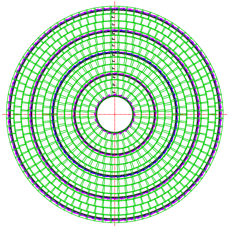
Figure II-3.3 R \phi projection view of the main tracker barrels (red) and disks (green).
