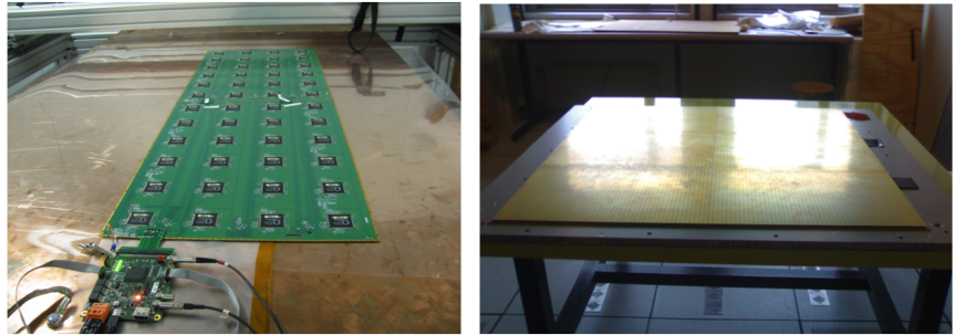
Figure III-3.17 An electronic slab made of two boards hosting each 24 ASIC and connected with a tiny connector. The interface DAQ board(DIF) is also shown (left) and the final 1 m 2 board.
