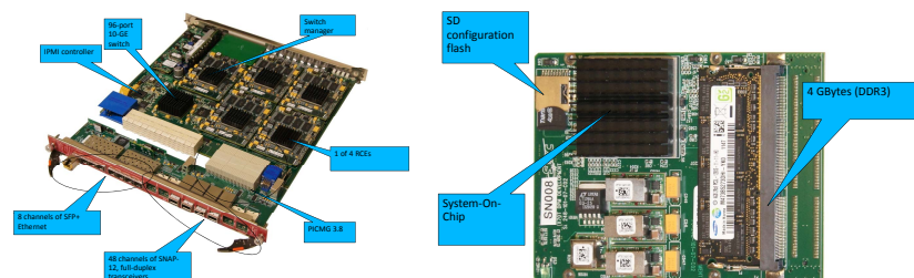
Figure II-9.4 ATCA Reconfigurable Cluster Element (left) and RCE daughter module (right)
