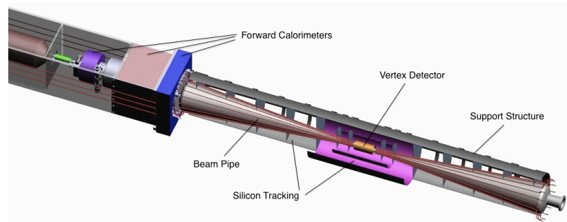
Figure III-5.19 The interaction region of ILD.
