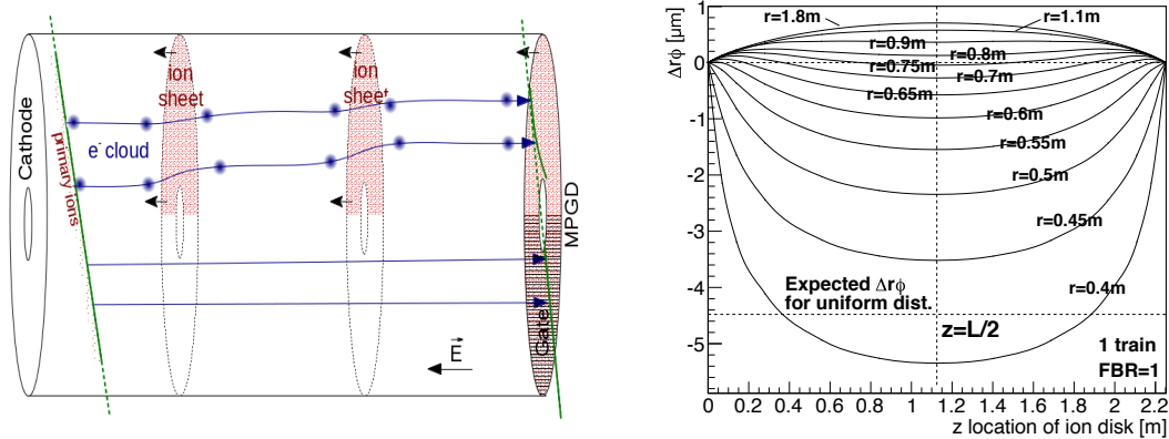
Figure III-2.15. (Left) Effects of the ion disks on the electrons inside the TPC volume. The effects without (top half of the figure) and with (bottom half of the figure) are compared. (Right) Expected distortions in r - \phi as simulated for a disk of charge located inside the TPC drift volume at different z -values, for a range of radii. For more details see the text.
