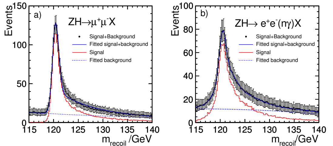
Figure III-6.6. Results of the model independent analysis of the Higgs-strahlung process e^+e^- \rightarrow hZ in which a) Z \rightarrow \mu^+\mu^- and b) Z \rightarrow e^+e^- (including the reconstruction of bremsstrahlung and FSR photons). The results are shown are for the P(e^+, e^-) = (+30\%, -80\%) beam polarisation.
