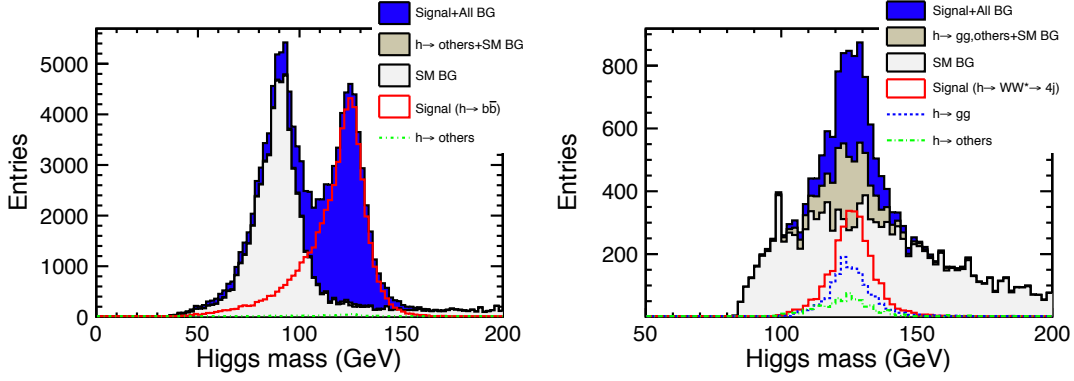
Figure III-6.11. Left: Reconstructed h \rightarrow b\bar{b} di-jet mass distribution after the b-tagging selection. Right: Reconstructed Higgs mass distribution in h \rightarrow WW^* fully hadronic decay channel. Both figures correspond to the DBD \mathcal{P}_{-80,+20} sample.
