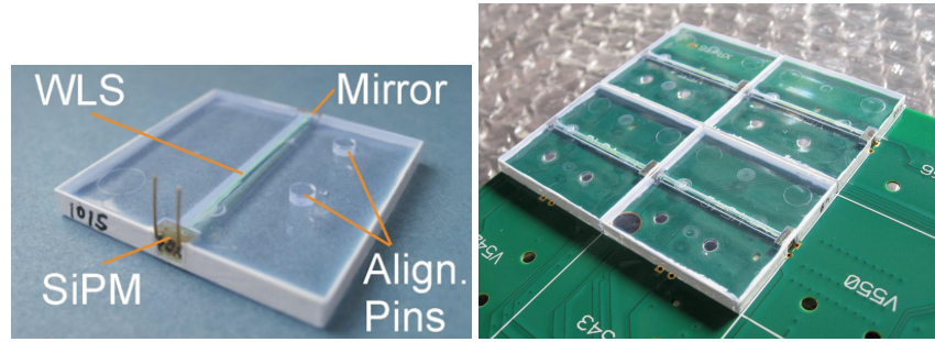
Figure III-3.15 The AHCAL scintillator tiles with embedded SiPMs, mounted on the readout PCB.
