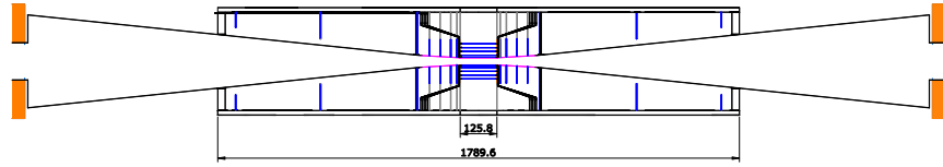
Figure II-2.1 Layout of the vertex and forward tracking region, including carbon-fibre support and forward cone. Dimensions are in mm
