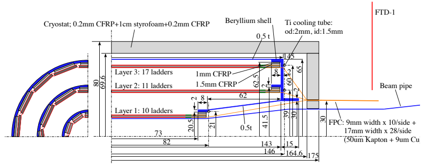
Figure III-2.7 Mechanical support structure of ILD vertex detector
