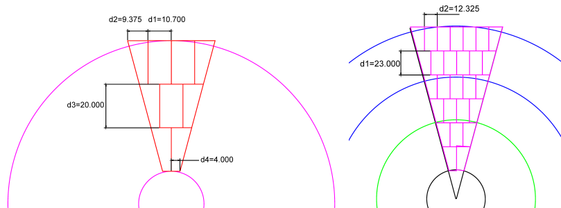
Figure II-2.5 Design of the reticule-based tiling for the innermost pixel disk (left) and for the disks at large z (right) with inner radii of 28 (black), 76 (green) and 117 (blue) mm and an outer radius of 166 mm.
