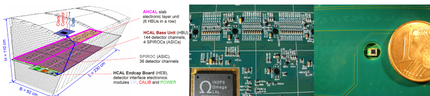
Figure II-4.23 Conceptual design of a barrel wedge instrumented with IRL planes (left), a HBU prototype (centre) with a MPPC surface-mounted on it (right).
