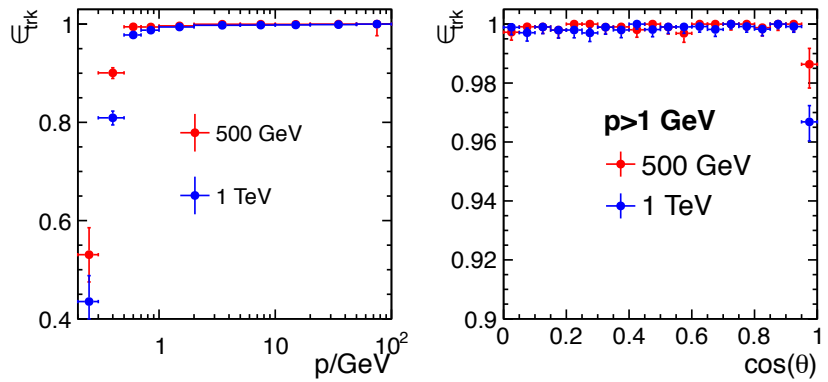
Figure III-6.2 Tracking Efficiency for t\bar{t} \rightarrow 6 jets at 500GeV and 1 TeV plotted against (left) momentum and (right) \cos\theta .
