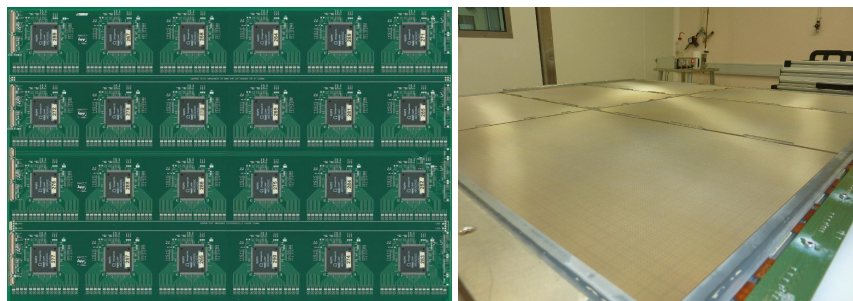
Figure II-4.18 One Active Sensor Unit (ASIC side) and the 1\text{ m}^2 prototype during assembly.
