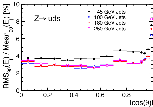
Figure III-6.4 Fractional jet energy resolution plotted against |\cos\theta| where theta is the thrust axis of the event.
