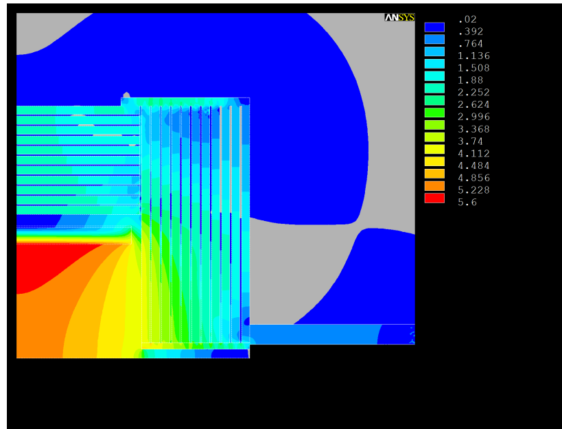
Figure II-6.2 :2D Axisymmetric showing B_{max} . Only a small portion of the air is displayed. The gray/blue boundary is the 200 G line.
