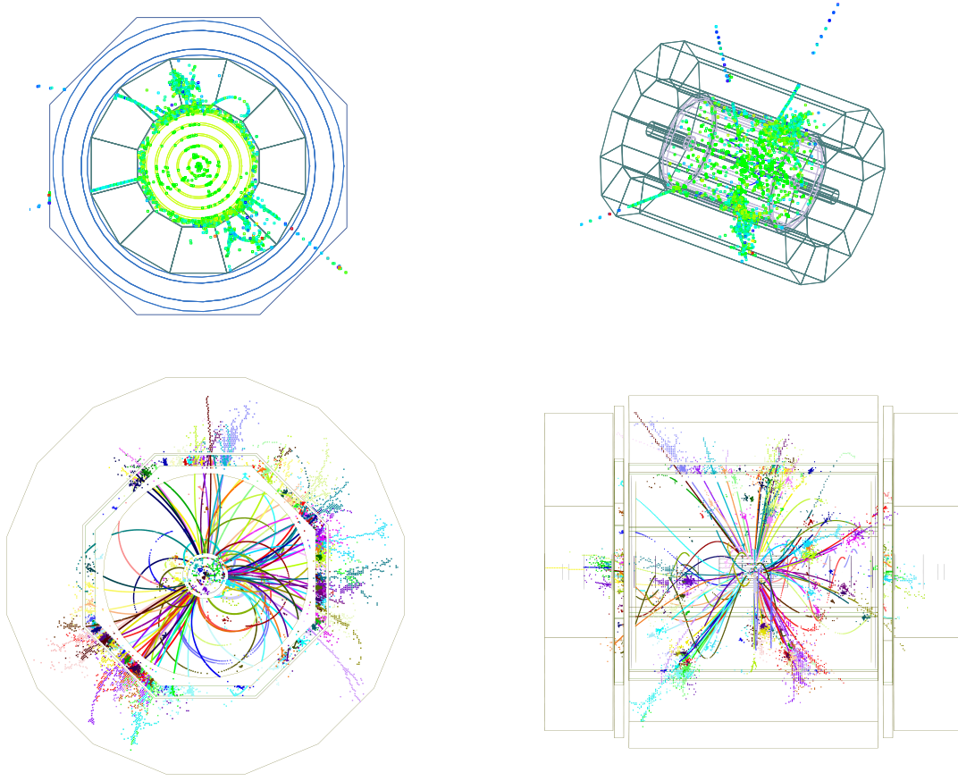
Figure I-1.2. Two event displays for: (up) e^+e^- \rightarrow Zh; Z \rightarrow \mu^+\mu^-; h \rightarrow b\bar{b} at 250 GeV from SiD and (down) e^+e^- \rightarrow t\bar{t}; t\bar{t} \rightarrow 6q; h \rightarrow b\bar{b} from ILD at 1 TeV.
