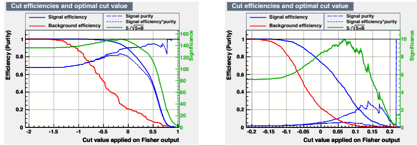
Figure II-11.9 Efficiency and significance curves vs. cuts on the MVA Fisher discriminant output for the h \rightarrow b\bar{b} (left) and c\bar{c} selections (right).
