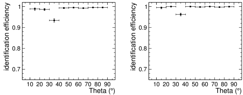
Figure II-10.6 Particle identification efficiency for 10 GeV photons (left) and 100 GeV photons (right) as a function of the angle \theta .
