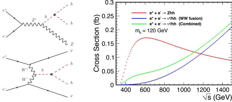
Figure III-6.16. Left: The Feynman diagrams involving the trilinear Higgs self-coupling for the two processes: e^+e^- \rightarrow Zh h (top) and e^+e^- \rightarrow \nu\bar{\nu}hh (bottom); Right: Cross section for these two processes as a function of \sqrt{s} for m_h=120 GeV. The blue dotted line shows the cross section for e^+e^- \rightarrow \nu\bar{\nu}hh from the WW fusion process alone, while the green dotted line shows the sum of the WW fusion contribution and the contribution from e^+e^- \rightarrow Zh h \rightarrow \nu\bar{\nu}hh .
