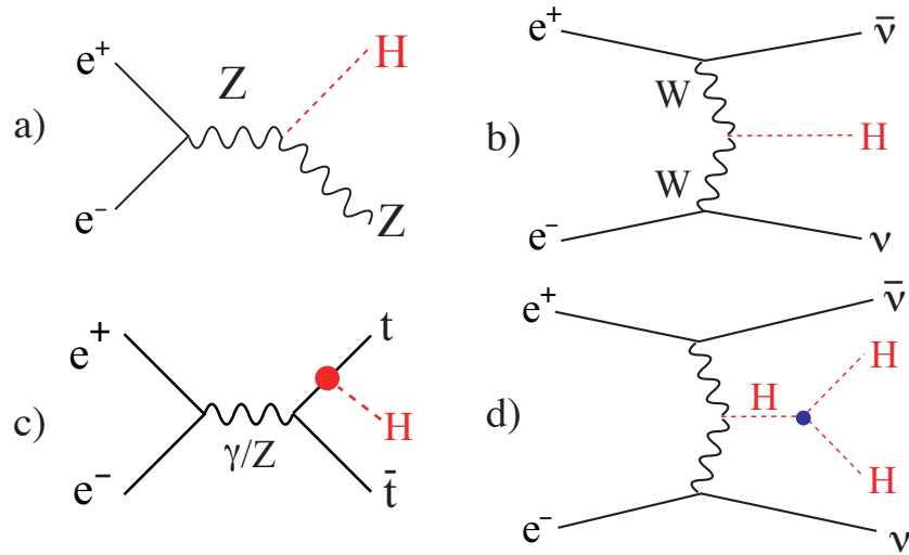
Figure I-1.1 Representative Feynman diagrams for the major Higgs production processes at the ILC: (a) e^+e^- \rightarrow Zh ; (b) e^+e^- \rightarrow \nu\bar{\nu}h ; (c) e^+e^- \rightarrow t\bar{t}h ; (d) e^+e^- \rightarrow \nu\bar{\nu}hh .
