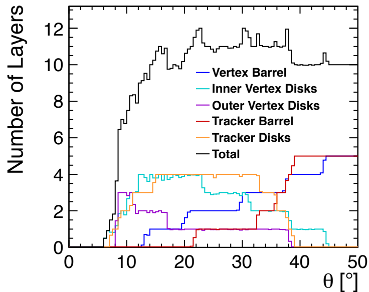
Figure II-3.2 The coverage of the SiD tracking system as a function of the polar angle \theta .
