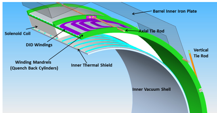
Figure II-6.1 Magnet section showing its principal elements.
