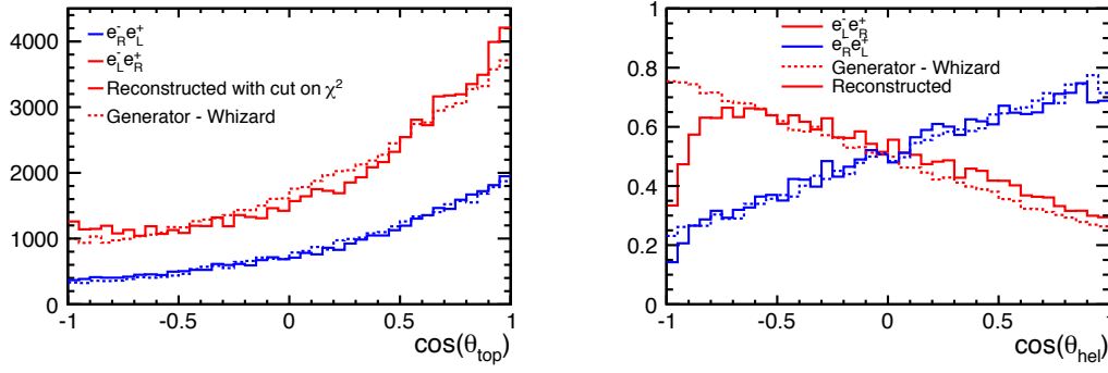
Figure III-6.18. Left: Reconstruction of the direction of the t quark for two different beam polarisations. The plot shown is an update of the one presented in [440]. Note that the figure does not include background, however, it is known from the studies in [387] that the background is negligible. Right: Generated and reconstructed distribution of the helicity angle \cos\theta_{hel} .
