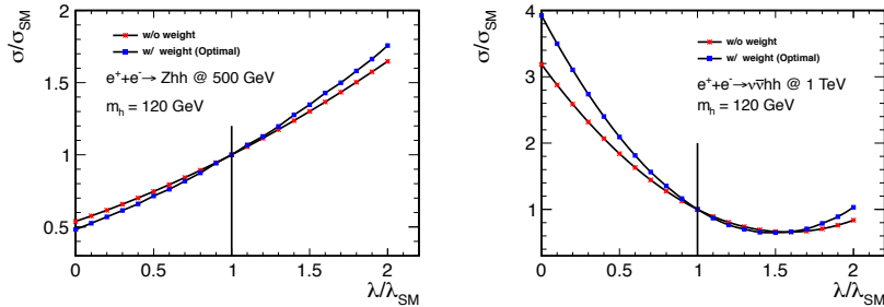
Figure III-6.17 The sensitivity of the Higgs self-coupling for the two processes: e^+e^- \rightarrow Zh h (left) and e^+e^- \rightarrow \nu\bar{\nu}hh (right). The red ones are without weighting and the blue ones are with the optimal weighting described in the reference [435].
