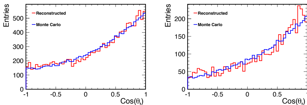
Figure III-6.15. Distribution of the true (blue curve) and reconstructed (red curve) polar angles of the identified top quark in fully-hadronic t\bar{t} events. The expected contributions from events with the wrong charge have been subtracted from the observed distribution. Left plot: \mathcal{P}_{-100,+100} ; right plot: \mathcal{P}_{+100,-100} . Both plots assume L = 250 \text{ fb}^{-1} .
