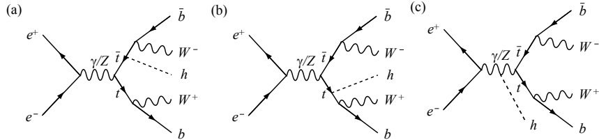
Figure I-2.6 Feynman diagrams for the e^+e^- \rightarrow t\bar{t}h process.
