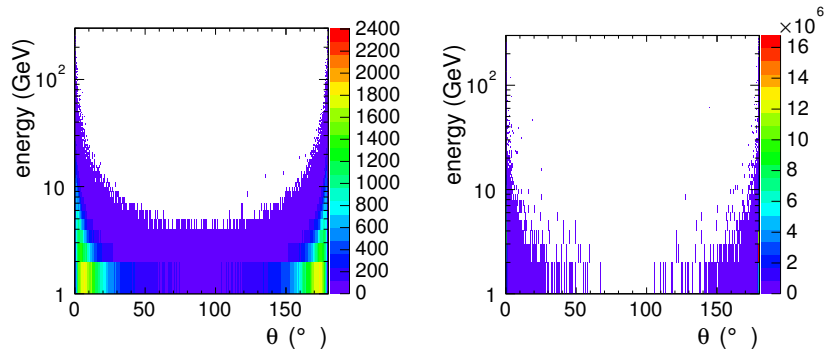
Figure II-10.5 Kinematic properties of the machine-induced backgrounds from \gamma\gamma \rightarrow hadrons processes (left) and from incoherent pairs (right) at 1 TeV.
