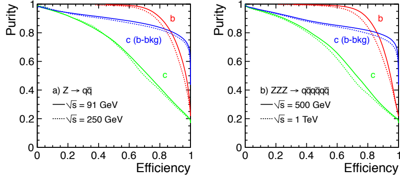
Figure III-6.5 Flavour tagging performance plots for (a) Z \rightarrow q\bar{q} samples at \sqrt{s} = 91 GeV and 250 GeV, and (b) ZZZ \rightarrow q\bar{q}q\bar{q}q\bar{q} samples at \sqrt{s} = 500 GeV and 1 TeV.
