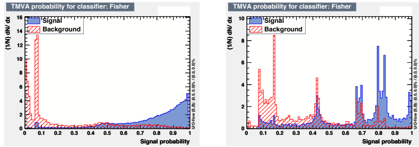
Figure II-11.8 Probability distributions for selecting Higgs boson decays to b\bar{b} (left) and c\bar{c} (right) from the Fisher Discriminant.
