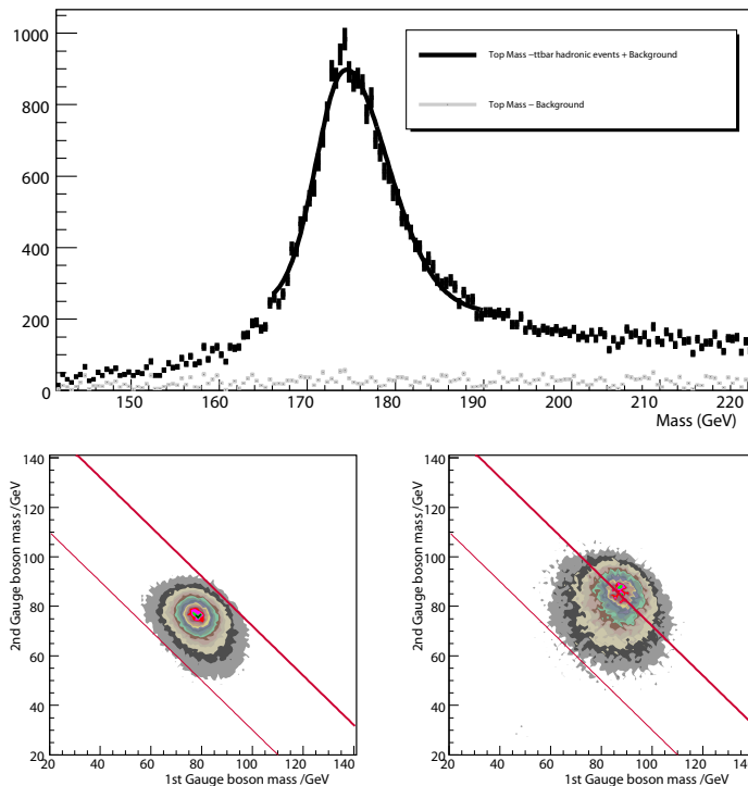
Figure II-11.2 Top analysis: Distribution of the top invariant mass after kinematic fitting (top). Chargino/neutralino analysis: The reconstructed boson masses from the four jets, selecting chargino events with a pure chargino signal (bottom left); and a pure neutralino signal (bottom right). The region between the two straight lines indicates the allowed chargino selection window.
