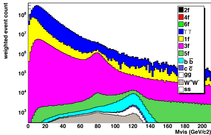
Figure II-11.7 Visible mass distributions for the backgrounds and \nu_e \bar{\nu}_e h events for the various Higgs decay modes.
