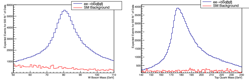
Figure II-11.13 Mass distribution of the W boson candidates (left) and top quark candidates (right).
