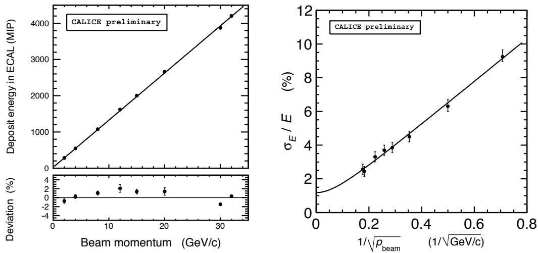
Figure III-3.10. Left: Response curve for the physics prototype of the ScECAL prototype vs. beam energy, with the deviation from a linear behaviour shown in the bottom part of the plot. The linearity is better than 2%. Right: Measured energy resolution of the physics prototype of the ScECAL prototype after temperature correction, for electrons in the energy range between 2 and 32 GeV. [310]
