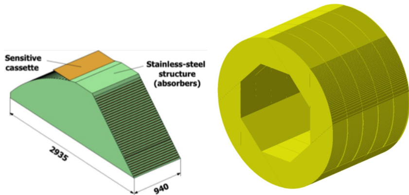
Figure III-5.4 Integration of the SD-HCAL structures.
