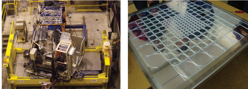
Figure II-4.21 CALICE test beam setup at CERN (left) and an active layer of the scintillator-SiPM prototype (right)
