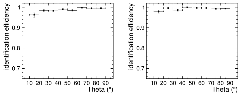
Figure II-10.8 Particle identification efficiency for 10 GeV muons (left) and 100 GeV muons (right) as a function of the angle \theta .
