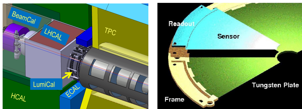
Figure III-3.24. Left: The very forward region of the ILD detector. LumiCal, BeamCal and LHCAL are carried by the support tube for the final focusing quadrupole QD0 and the beam-pipe. TPC denotes the central track chamber, ECAL the electromagnetic and HCAL the hadron calorimeter. Right: A half layer of an absorber disk with a sensor sector and front-end electronics.
