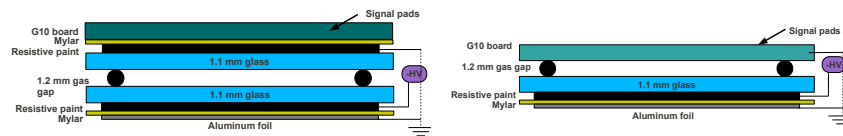
Figure II-4.8 Schematic of the RPC design with two glass plates (left) and one glass plate (right). Not to scale.
