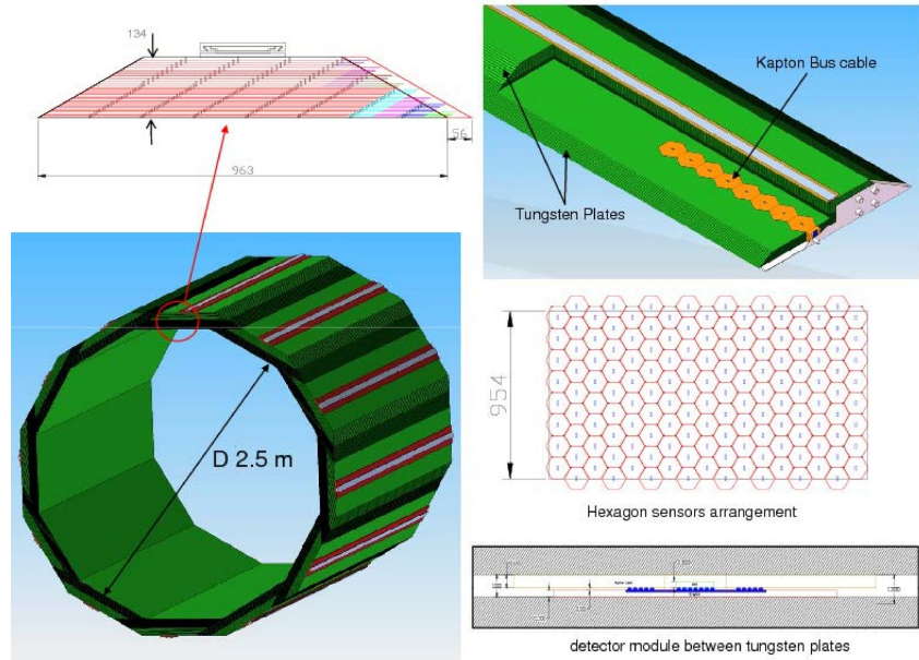
Figure II-4.1 Overall mechanical layout of the ECAL.
