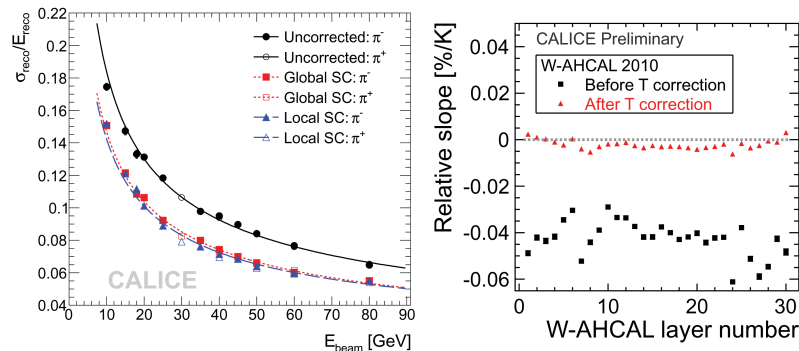
Figure II-4.22 Single pion resolution using simple energy sum and software compensation techniques (left) and slope of the SiPM response temperature dependence for AHCAL layers without and with temperature correction (right)
