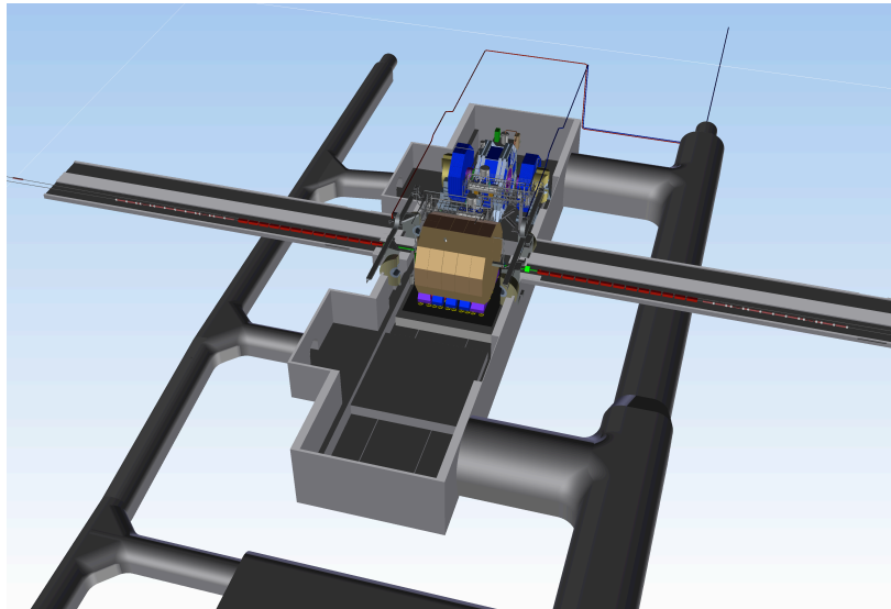
Figure III-5.17 The push-pull system at the ILC: ILD (front) and SiD (back) in the experimental hall (example of a mountainous ILC site).
