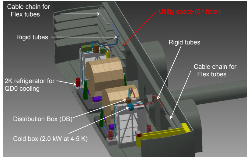
Figure I-2.14 Common detector cryogenic system (study) with the cold boxes placed on service racks close to the detectors.
