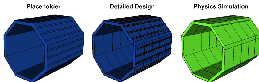
Figure III-5.12 Different models describe the ILD detector (this example: the ECAL barrel).
