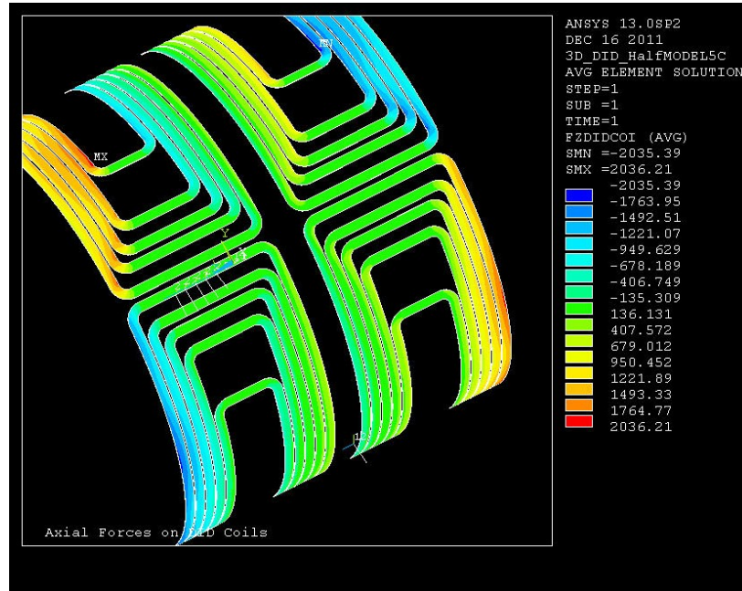
Figure II-6.3 DID coils showing axial forces; Only half of the coils are shown
