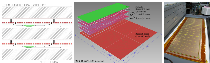
Figure II-4.17 Left: GEM DHCAL Concept. Centre: Drawing of the large-area GEM chamber. Right: Large-area GEM chamber under construction.
