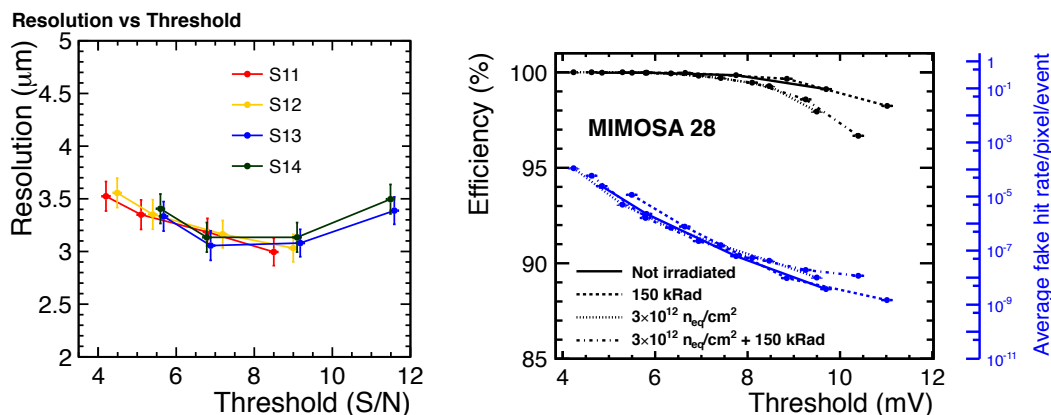
Figure III-2.2. Left: Single point resolution measured with a 18.4 \mu\text{m} pitch as a function of the discriminator threshold (the colours refer to different in-pixel circuits). Right: Measured variations of the minimum ionising particle (m.i.p.) detection efficiency and fake hit rate (fraction of pixel noise fluctuations above threshold) of the STAR sensor as a function of the discriminator threshold, before and after irradiation ( 150 \text{ kRad} , 3 \times 10^{12} \text{ n}_{eq}/\text{cm}^2 ) at a coolant temperature of 30^\circ\text{C} .
