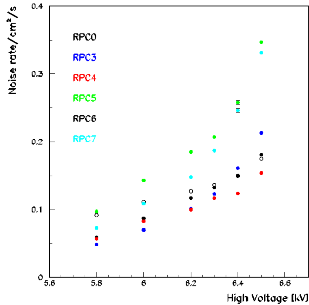
Figure II-4.16 Noise rate as function of high voltage for six different chambers. The threshold was set at the default value of 110 counts. The default high voltage setting was 6.2 kV.
