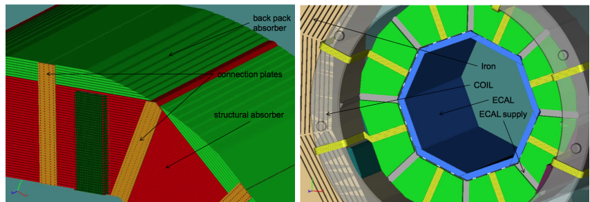
Figure III-5.3 Integration of the AH-CAL structures into the cryostat.
