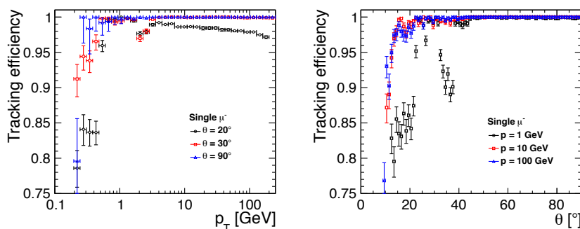
Figure II-3.5 Tracking efficiency for single muon events in SIDLO13 as function of the transverse momentum (left) and the polar angle (right).
