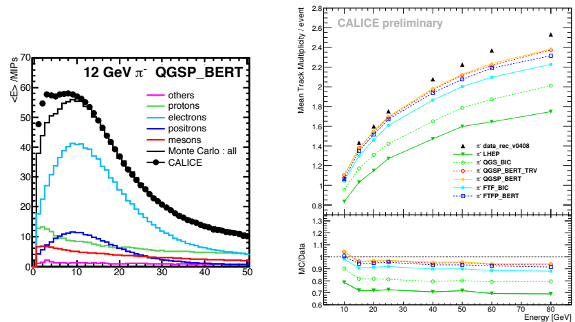
Figure I-2.4 Comparison of CALICE test beam data with simulations: longitudinal shower profile in the silicon tungsten ECAL, charged track multiplicity in the scintillator steel analogue HCAL.
