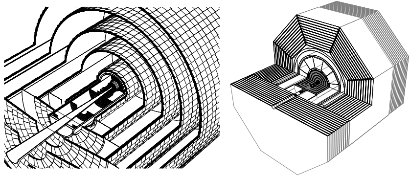
Figure II-10.3 Cutaway view of the tracking system as implemented in SIDLOI3 (left) and the complete detector (right). Some support and readout structures have been hidden to improve the visibility of the sensors (left) and the calorimeters.
