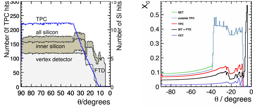
Figure III-6.1 (Left) Average number of hits for simulated charged particle tracks as a function of polar angle. (Right) Average total radiation length of the material in the tracking detectors as a function of polar angle.
