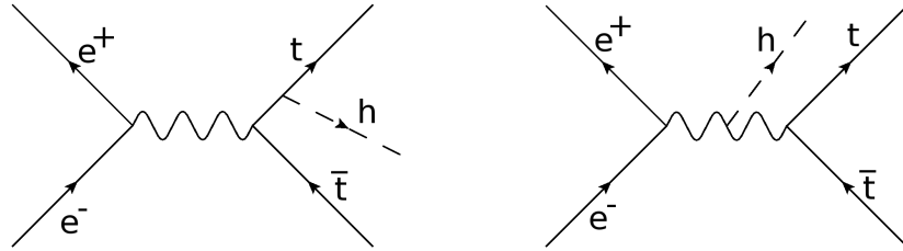
Figure II-11.3 Diagrams for t\bar{t}h production in e^+e^- collisions.
