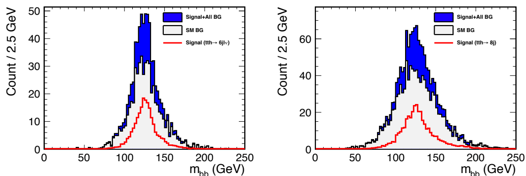
Figure III-6.14. Reconstructed h mass for the optimal jet combination of events passed the isolated lepton and Boosted Decision Tree cuts. Left: Semi-leptonic channel. Right: Fully hadronic channel. Both figures show the full DBD sample.
