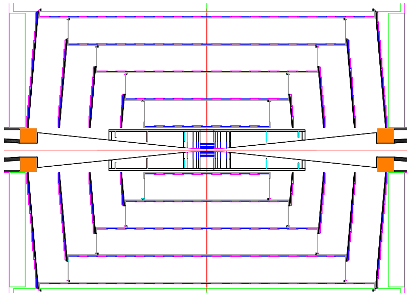
Figure II-3.1 r - z view of the vertex detector and outer tracker.
