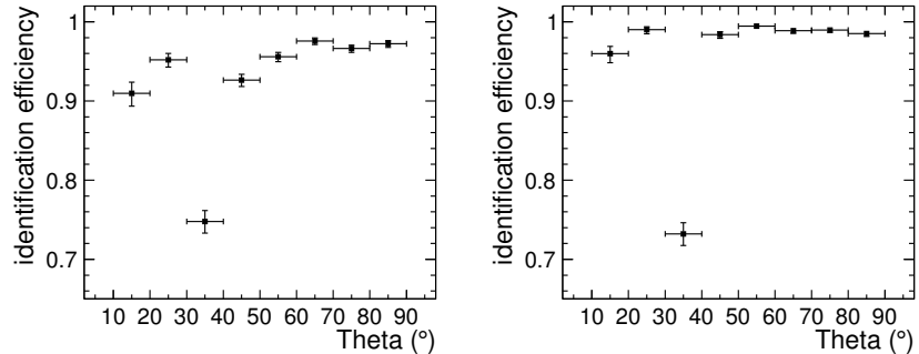
Figure II-10.7 Particle identification efficiency for 10 GeV electrons (left) and 100 GeV electrons (right) as a function of the angle \theta .
