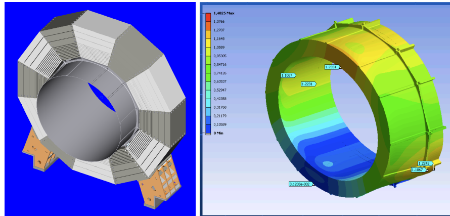
Figure III-5.2 Integration of the solenoid cryostat and the central yoke ring (left). FEM simulation of the cryostat deformations under its own mass and the mass of the barrel detectors (right).
