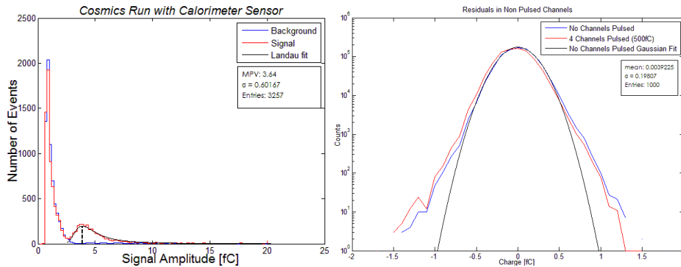
Figure II-4.4. Distribution of charge depositions in bonded sensor for cosmic ray triggered events (left). The MIP peak is clearly visible above the noise peak. Crosstalk test of bonded sensor (right). The charge distributions for all non-pulsed pixels are compared for a large pulse injection (red) and no pulse injection (blue). Also shown is a Gaussian fit with RMS 0.2 fC.
