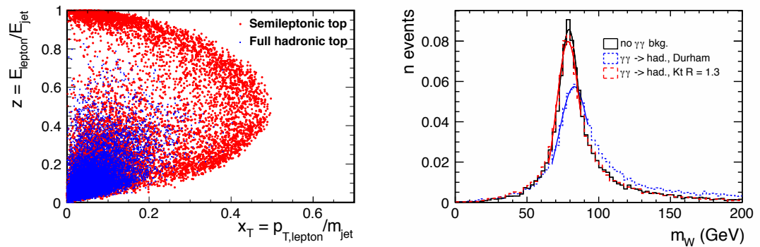
Figure III-6.9. Left: Distribution of variables x_T and z used to identify isolated leptons in semi-leptonic (red) and full hadronic (blue) top events. Right: Reconstructed di-jet mass distribution in e^+e^- \rightarrow WW \rightarrow \ell\nu qq . Black solid: Durham algorithm, no pile-up; Blue dotted: Durham algorithm, with pile-up; Red dashed: k_t algorithm, with pile-up.
