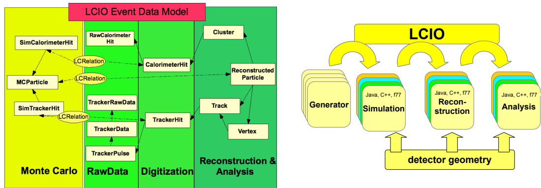
Figure I-2.7. Left: Schematic overview of the hierarchical event data model (EDM) of LCIO. Right: The common EDM and persistency scheme allow to exchange software tools even when they are written in different frameworks and languages.
