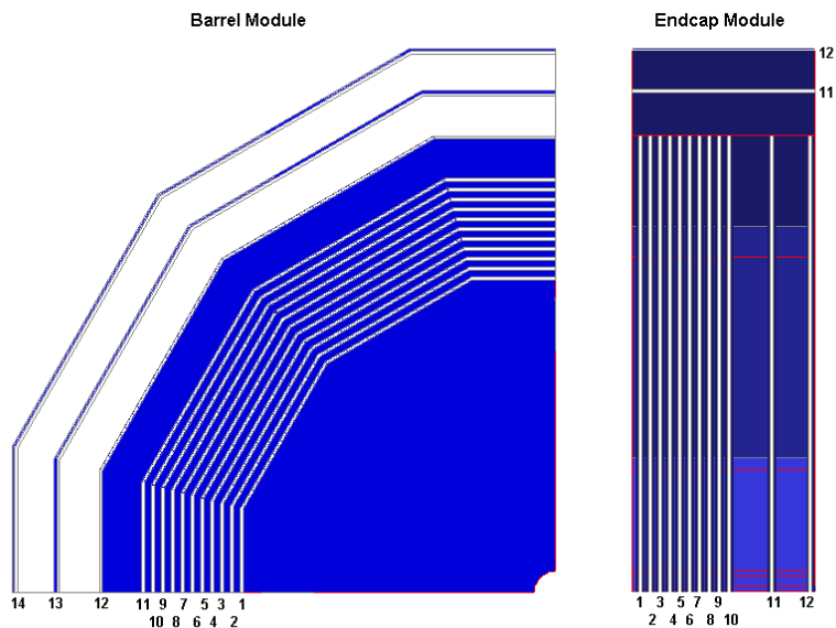
Figure III-4.1 Sensitive Layers of ILD Muon System/Tail Catcher
