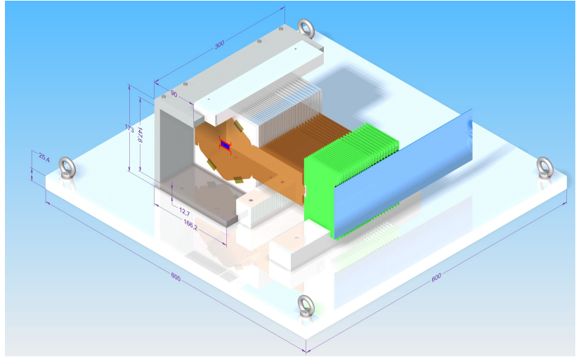
Figure II-4.5 Schematic of test module to be tested in a beam. The module has a width of one sensor and a depth of 30 layers. The Kapton cables attached to each sensor feed concentrator boards, which in turn are connected to a mother board.
