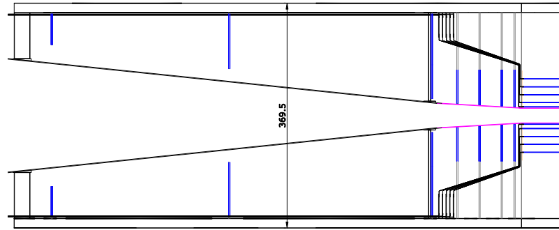
Figure II-2.2 R-z view of the vertex detector and its support structure. Cable routes are also shown with DC-DC converters located on the support structure near the end of the first set of pixel disks. Dimensions are in mm.
