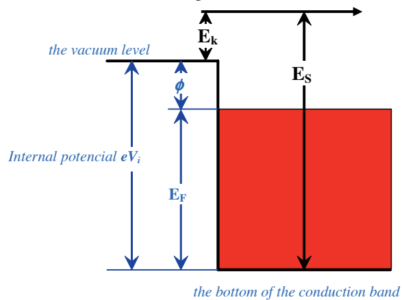
Figure 1: The energy level diagram.
