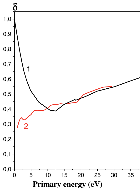
Figure 2: Total secondary electron emission yield of Cu at low electron primary energy E_p . 1. Initial part of Fig. 2 taken from the letter [3] for fully scrubbed Cu ( T=10 K). 2. Experimental data for Cu from Ref. [18] after applying heat in vacuum (taken at room temperature).
