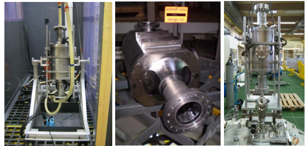
Figure 1: Left: Vertical BCP setup for heavy etching of the cavity surface (Courtesy Niowave Inc.). Middle: 4rod crab cavity preparation for the high temperature bake in UHV furnace. Right: High pressure water rinse setup at CERN.
