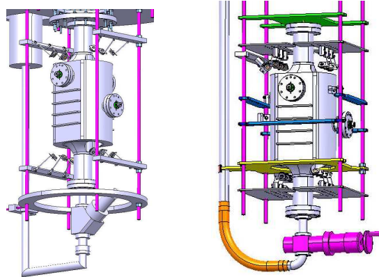
Figure 8: 4rod cavity integration layout for first cold RF measurements (left) and subsequent modification (right).
