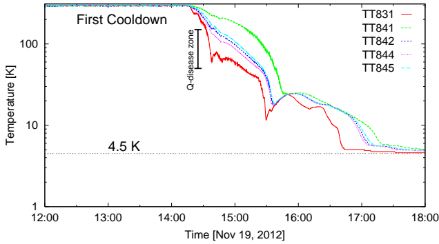
Figure 3: Temperature evolution during the first cool down of the 4Rod crab cavity.
