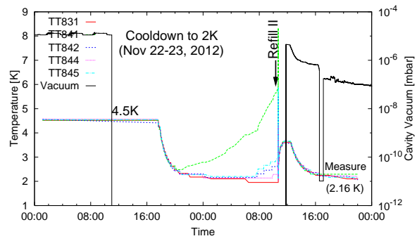
Figure 4: Temperature evolution during the cool down of the 4Rod crab cavity to 2 K. A Helium refill was necessary to maintain sufficient liquid level in the short cryostat.
