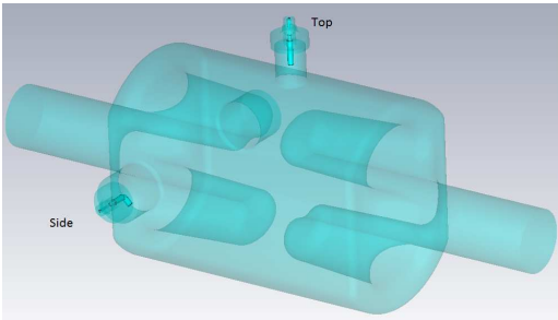
Figure 6: Input and pickup probe configuration for appropriate coupling required in the vertical tests.
