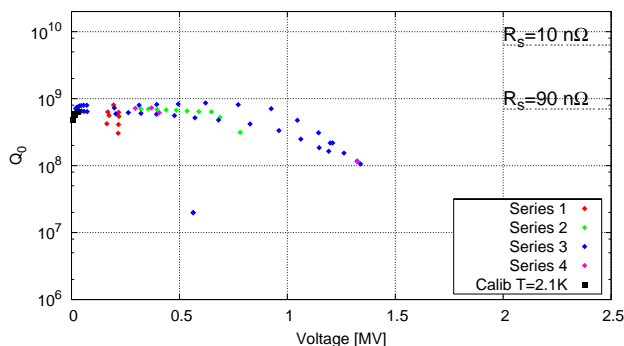
Figure 7: Measured cavity quality factor as a function of deflecting voltage in the cavity.
