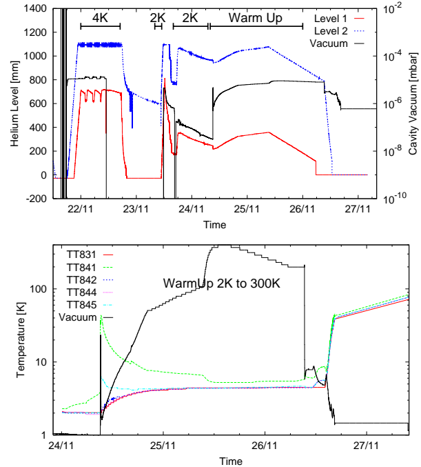
Figure 5: Helium liquid level (top) and temperature evolution (bottom) at 2 K and the warm up of the cavity.
