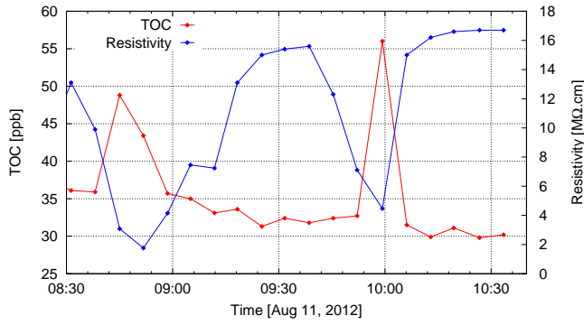
Figure 2: Total organic content and resistivity of the water during the high pressure water rinsing of the cavity.
