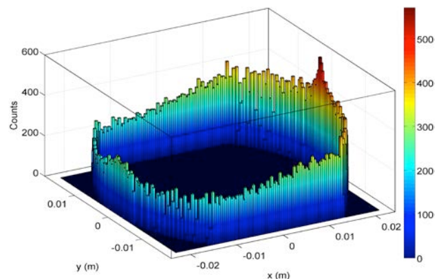
Figure 4: Distribution of total photon absorption sites.
