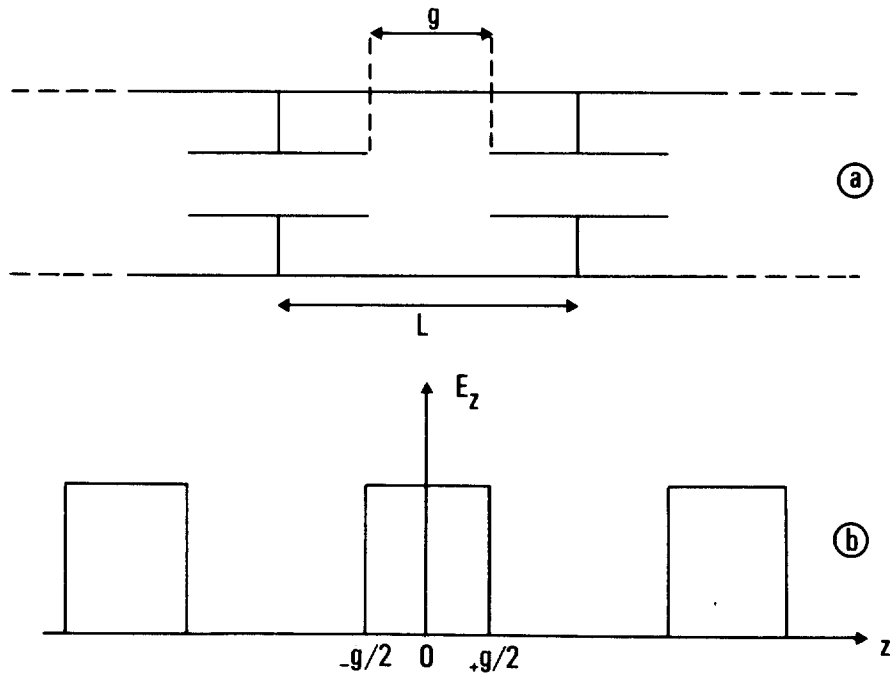
Fig. 13 - Approximate field pattern in a drift tube accelerator
