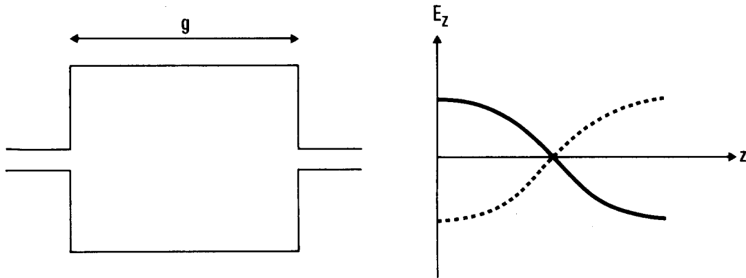
Fig. 14 - TM_{011} mode in a pill-box cavity
