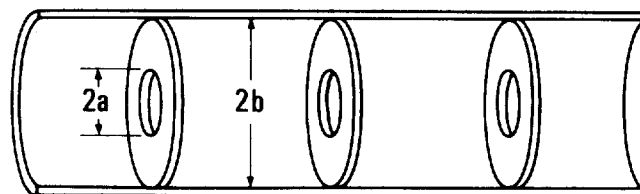
Fig. 6 - Disk-loaded structure
