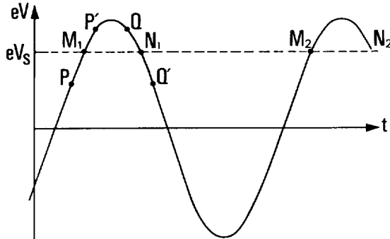
Fig. 20 - Particle phases relative to the RF field
