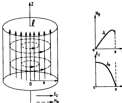
Fig. 15 - TM_{010} mode in a pill-box cavity
