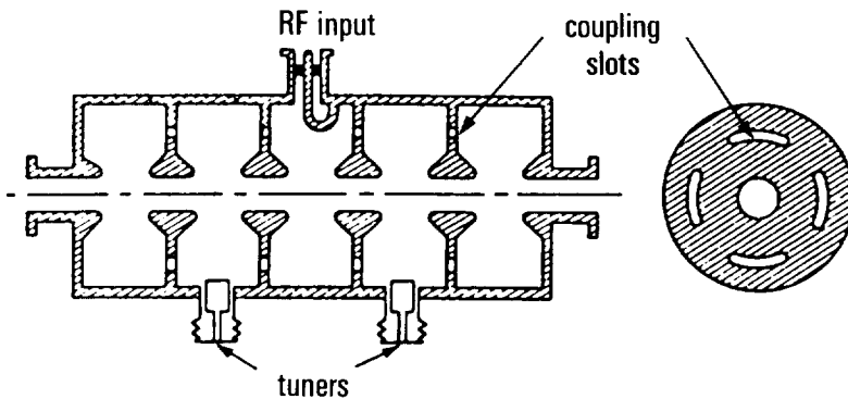
Fig. 8 - Nose cone structure
