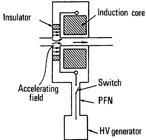
Fig. 10 - Linear induction accelerator module
