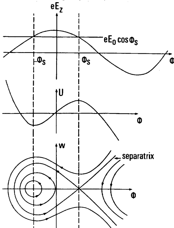
Fig. 21 - Phase stability graphs
