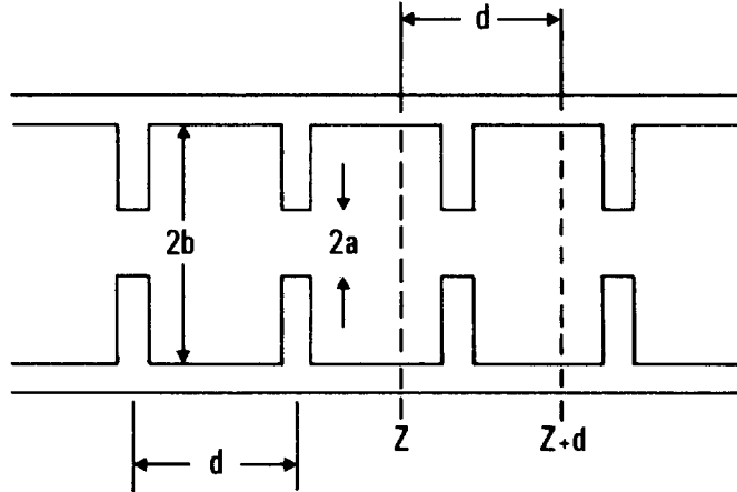
Fig. 17 - Periodic loaded structure
