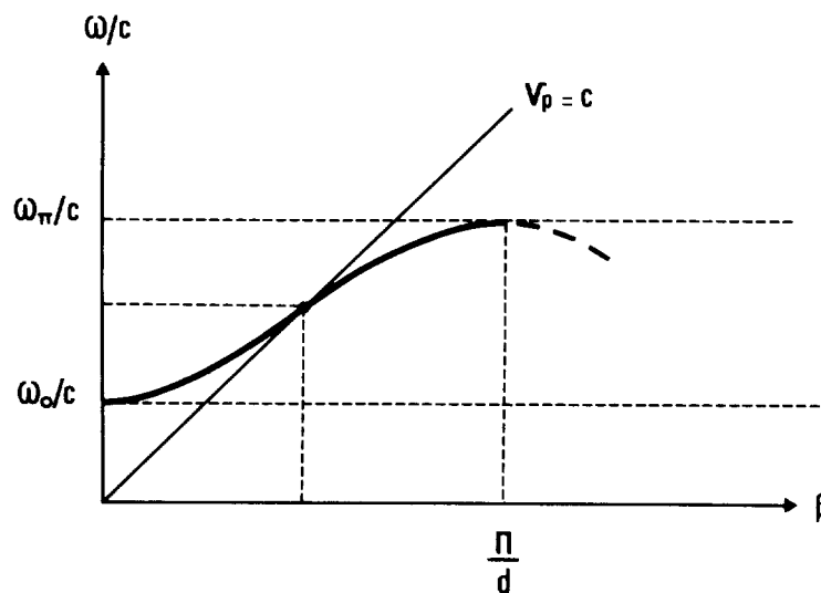
Fig. 19 - Operating point for v_p = c
