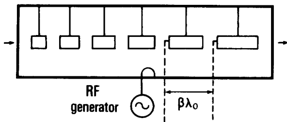
Fig. 5 - ALVAREZ type structure
