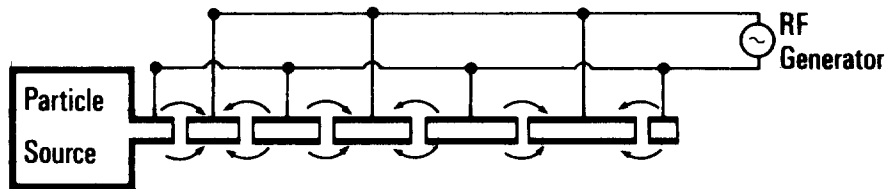
Fig. 2 - WIDEROE type accelerator
