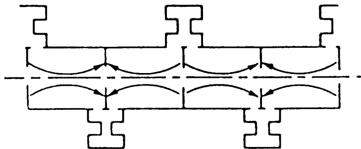
Fig. 9 - Side coupled structure
