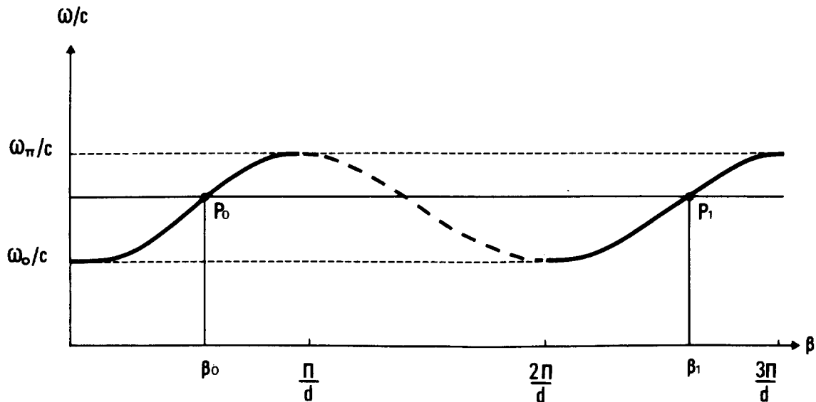
Fig. 18 - Brillouin diagram for a slow wave structure
