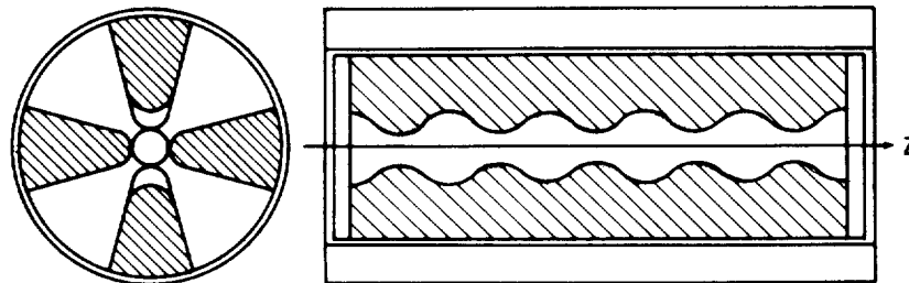
Fig. 11 - Schematic drawing of an RFQ resonator
