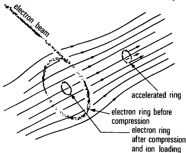
Fig. 12 - Principle of the Electron Ring Accelerator (ERA)
