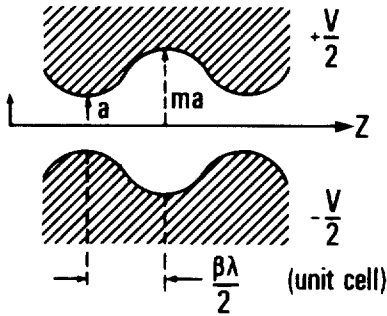
Fig. 23 - Modulated pole shapes in an RFQ
