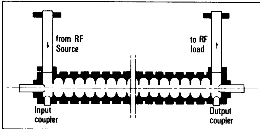
Fig. 7 - Travelling wave accelerating structure
