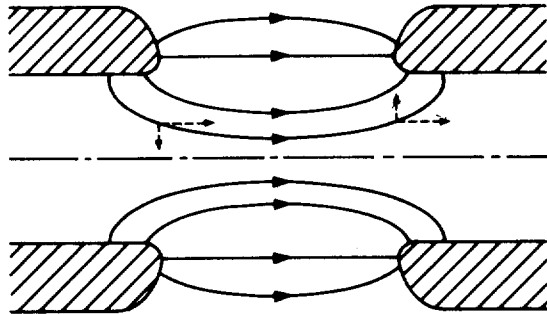
Fig. 22 - Field pattern in the gap of a drift tube accelerator
