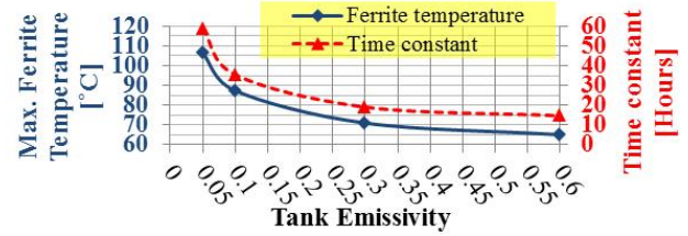
Figure 3: Predicted max. ferrite temperature, for a power deposition of 45.5 W/m, versus tank emissivity. The time-constant for cool-down of the ferrite yoke is also shown.
