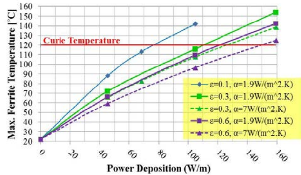
Figure 4: Predicted max. ferrite temperature versus total power deposition per m length of ferrite yoke, for various emissivities of the inside of the tank and convection ( \alpha ).
