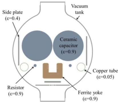
Figure 2: Slice through cross-section of an MKI magnet.
