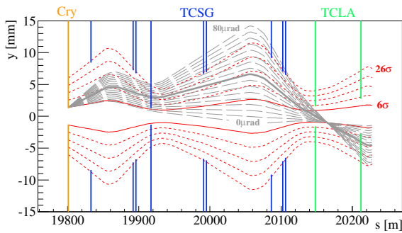
Figure 2: Same notation as in Fig. 1, but for the vertical plane.
