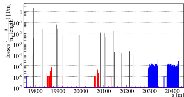
Figure 3: Local cleaning inefficiency in the IR7, in case of standard collimation. Losses on: collimators (grey bars), warm magnets (red bars), superconducting magnets in the DS (blue bars)
