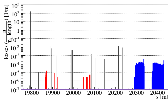
Figure 5: Local cleaning inefficiency in the IR7, in case of crystal at the TCP in amorphous orientation. And same notation as in Fig. 3
