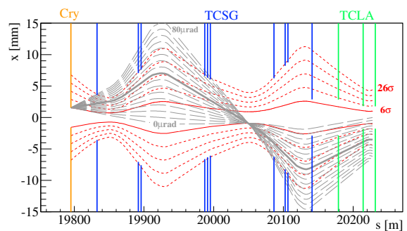
Figure 1: From 6\sigma to 26\sigma beam envelope with steps of 5\sigma (red lines), trajectory of particle experienced a kick from 0\mu\text{rad} to 80\mu\text{rad} with steps of 5\mu\text{rad} (gray lines), versus longitudinal position in IR7. Orange line: crystal aperture, blue lines: projection on the plane of interest of the secondary aperture, green lines: projection on the plane of interest of the absorbers aperture.
