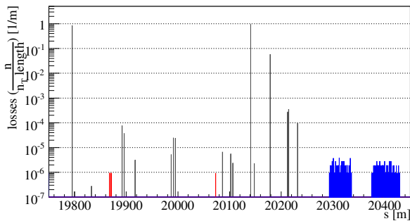
Figure 4: Local cleaning inefficiency in the IR7, in case of crystal at the TCP in channeling orientation. And same notation as in Fig. 3
