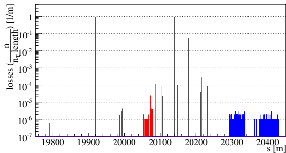
Figure 6: Local cleaning inefficiency in the IR7, in case of crystal at the TCSG in channeling orientation. And same notation as in Fig. 3
