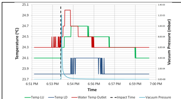
Figure 5: Test 1 temperature profiles captured by the upstream (LU) and downstream (LD) left jaw temperature sensors and by the water outlet temperature sensor. Also, vacuum pressure profile for Test 1. Impact at 6.53.51 PM.
