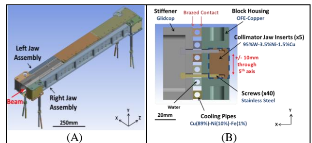
Figure 1: A horizontal tertiary collimator (TCTH). (A) 3D model. (B) Detailed cross-section in the x-y plane of the left jaw assembly.
