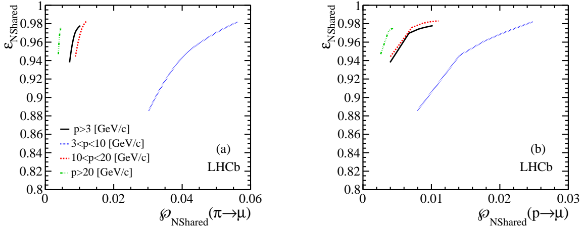
Figure 10. Muon efficiency \epsilon_{\text{NShared}} as a function of the pion and proton misidentification probabilities. The average values, for all particles with p > 3 \text{ GeV}/c , are shown with a black line, compared to the three momentum ranges separately, as for figure 7.
