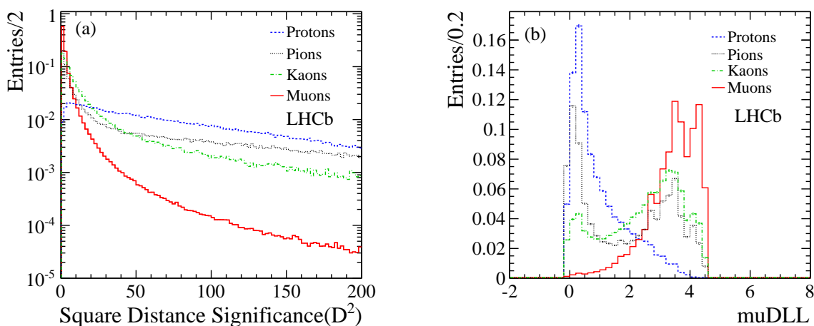
Figure 3. Average square distance significance distributions for muons, protons, pions and kaons (a) and the corresponding muDLL distributions (b).
