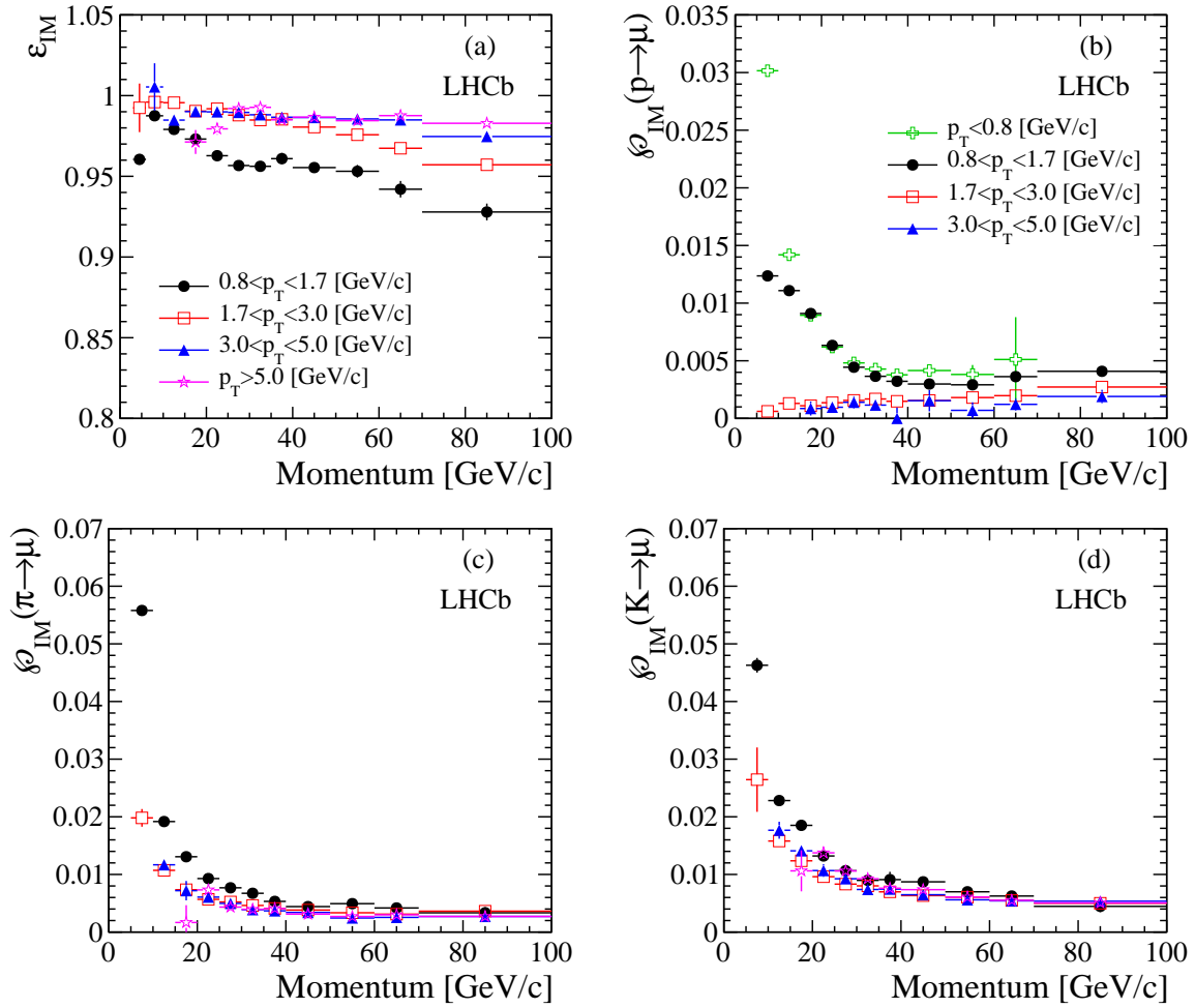
Figure 5. IsMuon efficiency and misidentification probabilities, as a function of momentum, in ranges of transverse momentum: \varepsilon_{IM} (a), \rho_{IM}(p \rightarrow \mu) (b), \rho_{IM}(\pi \rightarrow \mu) (c) and \rho_{IM}(K \rightarrow \mu) (d).
