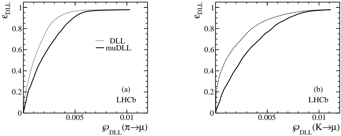
Figure 9. Average efficiency \epsilon_{\text{DLL}} as a function of the pion (a) and kaon (b) misidentification probabilities for particles with momentum in the range p > 3 \text{ GeV}/c . The dotted lines show the DLL performance, while the muon DLL performance is shown with a solid line.
