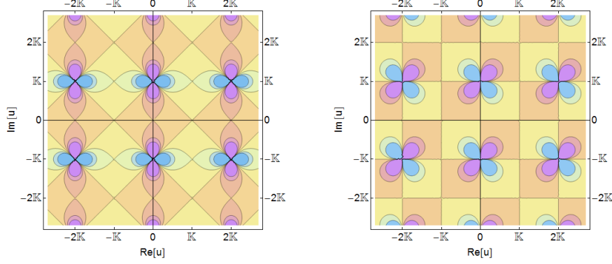
Figure 7. Real and imaginary parts of the Lamé potential, \text{sn}^2(u|1/2) .
