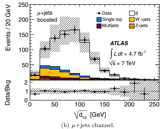
FIG. 8 (color online). The first k_t splitting scale, \sqrt{d_{12}} , of the large-radius jet from the hadronically decaying top quark in (a) the e +jets and (b) the \mu +jets channels, after the boosted selection, except the requirement \sqrt{d_{12}} > 40 \text{ GeV} . The shaded area indicates the total systematic uncertainties.
