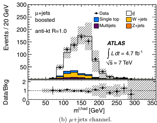
FIG. 7 (color online). The mass of the large-radius jet from the hadronically decaying top quark, m^{t,\text{had}} , in (a) the e +jets and (b) the \mu +jets channels, after the boosted selection, except the requirement m^{t,\text{had}} > 100 \text{ GeV} . The shaded area indicates the total systematic uncertainties.
