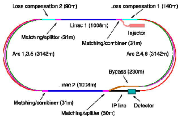
Figure 2: Conceptual layout of the LHeC ERL
