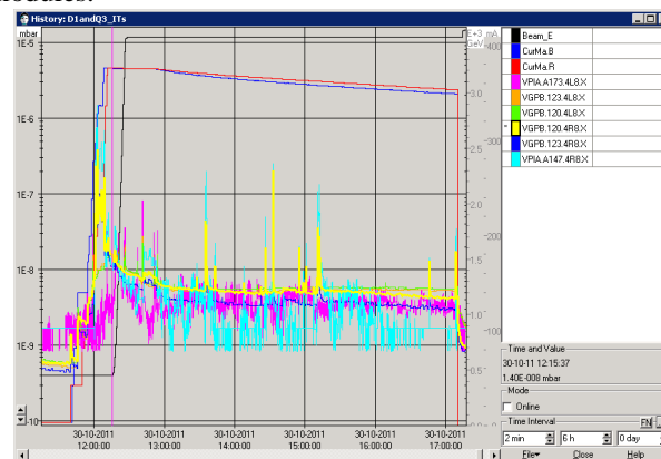
Figure 8: Typical pressure spikes observed in LSS 2 and LSS8 induced by sparking inside VAMTF module (fill 2267).
