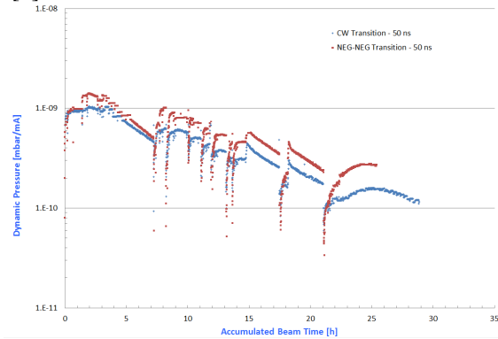
Figure 2: Dynamic pressure increase due to electron cloud observed at the stand alone magnets extremities as a function of beam time.
