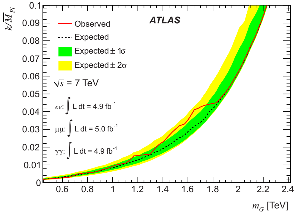
Figure 4. The RS results interpreted in the plane of k/\overline{M}_{Pl} versus graviton mass. The region above the curve is excluded at 95% CL.
