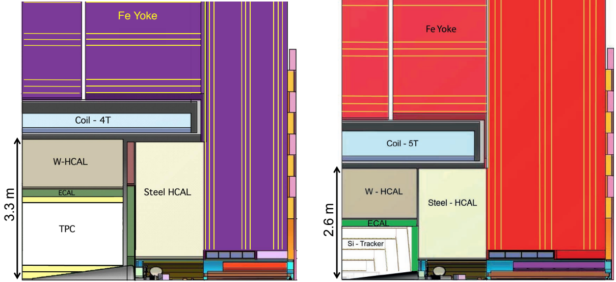
Fig. 4.2: Longitudinal cross section of the top quadrant of CLIC_ILD (left) and CLIC_SiD (right).
