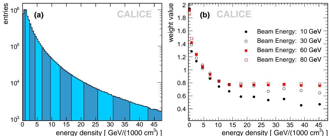
Figure 5. (a) Distribution of the cell energy density in the AHCAL for 40 GeV pion showers. The energy density is given by the uncorrected reconstructed energy in that cell, divided by the corresponding absorber volume. The different energy density bins used in the analysis are indicated by colour shades. (b) Optimal weights as a function of energy density for different beam energies, determined without constraints of a specific functional form in the first iteration of the minimisation.
