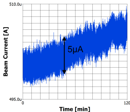
Figure 3: H_3^+ beam intensity measured over 2 hours with the Faraday Cup. The beam current amounts to \sim 500 \mu A H_3^+ .
