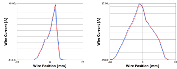
Figure 4: H_3^+ horizontal and vertical beam profile measured with the Wire Scanner immediately after the spectrometer.
