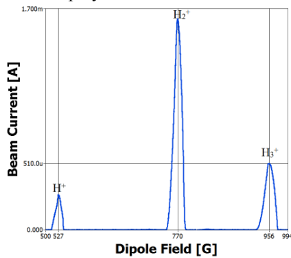
Figure 2: Proton source spectrum measured with an FC during the dipole ramp with a slit opening of 29 mm.
