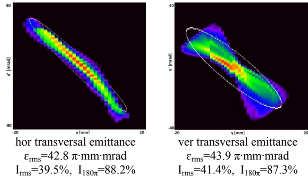
Figure 5: H_3^+ transverse emittance in both planes. The ellipse defining the 180 \pi \cdot mm \cdot mrad is visualized.
