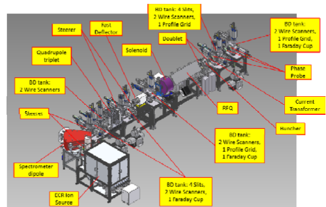
Figure 1: Layout of the final ITS
