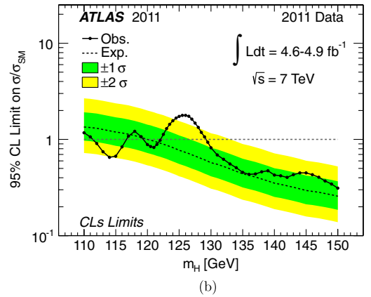
FIG. 4 (color online). The observed (solid line) and expected (dashed line) 95% CL combined upper limits on the SM Higgs boson production cross section divided by the SM expectation as a function of m_H , (a) in the full mass range considered in this analysis and (b) in the low mass range. The dotted curves show the median expected limit in the absence of a signal and the green and yellow bands indicate the corresponding \pm 1\sigma and \pm 2\sigma intervals.
