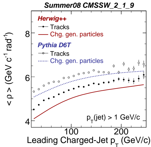
Figure 7.15: SUMMER08: Average event-by-event median ratio of jet p_T and jet area shown as a function of the leading charged-jet p_T . Predictions are from HERWIG (filled symbols) and from PYTHIA (hollow symbols). Charged k_{\perp} jets with p_T > 1 GeV/ c selected.
