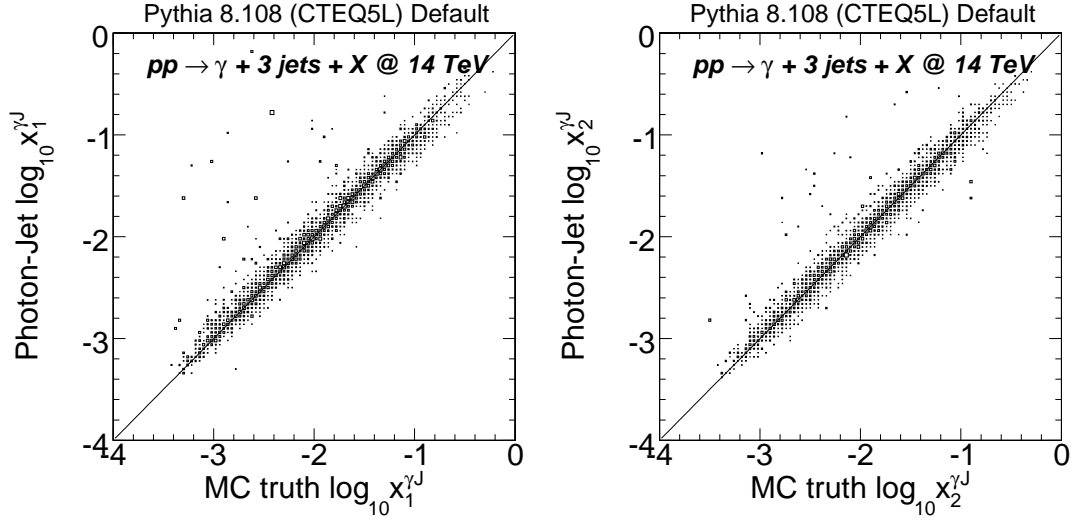
Figure 5.23: Proton momentum fractions entering the prompt photon production process determined with the photon-jet pair (Eq. 5.22) shown as a function of Monte Carlo truth. Correlation predictions shown for proton 1 (left) and proton 2 (right).
