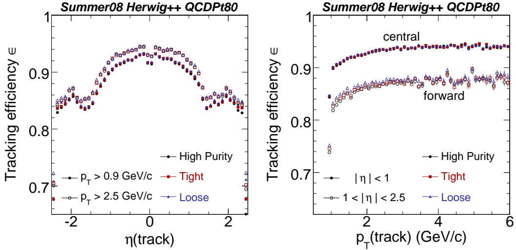
Figure 6.2: Global tracking efficiency distributions to reconstruct charged particles as high purity, tight or loose tracks. The efficiency is shown for p_T thresholds 0.9 GeV/ c and 2.5 GeV/ c as a function of pseudorapidity (left) and for |\eta| < 1 (“central”) and 1 < |\eta| < 2.5 (“forward”) as a function of transverse momentum (right). Note that the global tracking efficiency is not independent of p_T in the region 0.9 \text{ GeV}/c < p_T(\text{track}) < 1.5 \text{ GeV}/c (cf. Sec 7.3.2).
