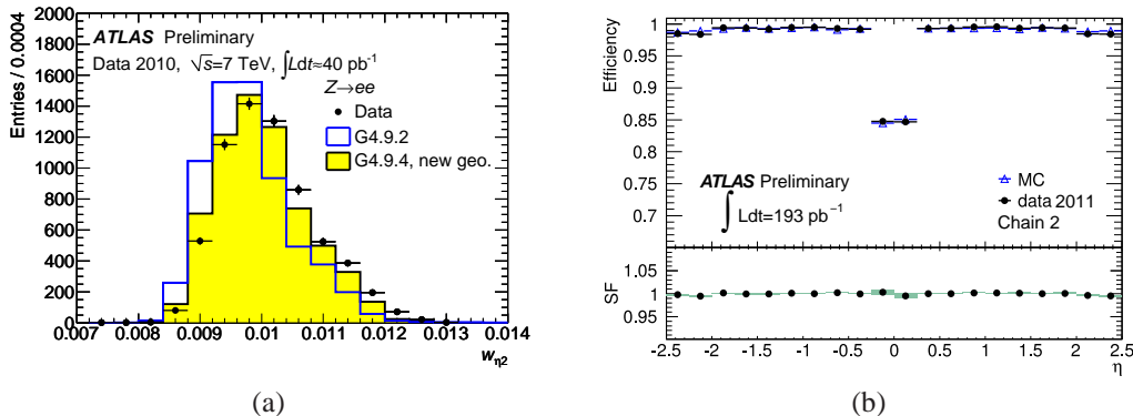
Fig. 3. – The lateral width of the shower in the middle layer of the electromagnetic calorimeter in data and simulation (a) [12]; and the efficiency for a muon candidate to be successfully reconstructed in the muon spectrometer and associated to an ID track, defined with respect to an ID track (b) [13]. The bottom plot in fig. (b) shows the ratio of measured and predicted efficiency.
