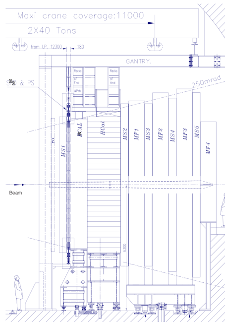
Figure 1 Structure of the LHCb calorimeters.
