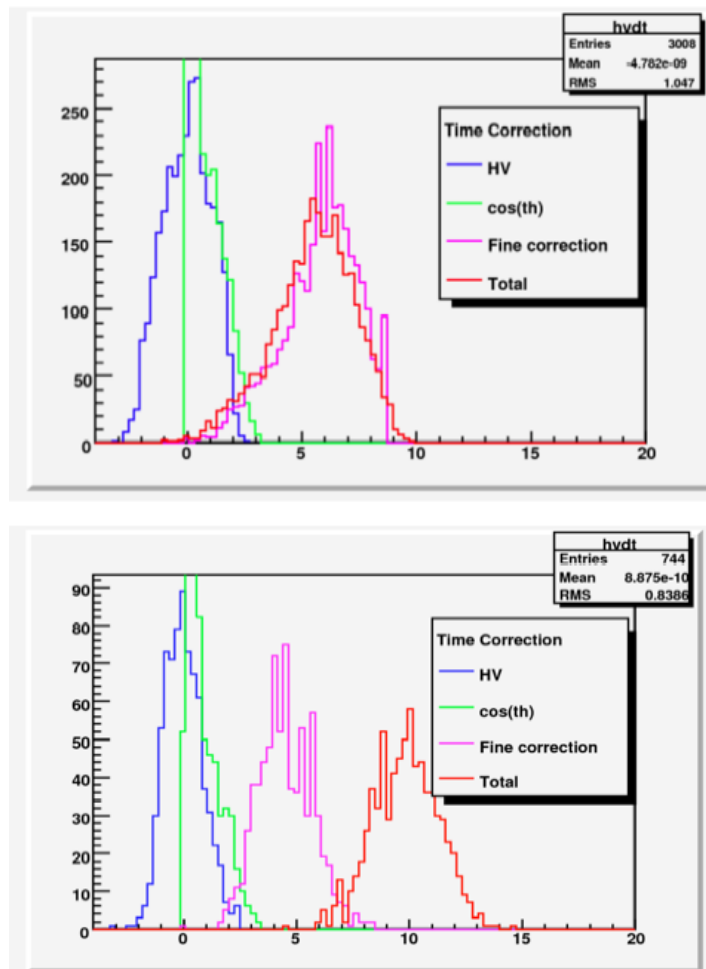
Figure 17 Different timing component contributions to the timing from ECAL (top) and HCAL detector (bottom).
