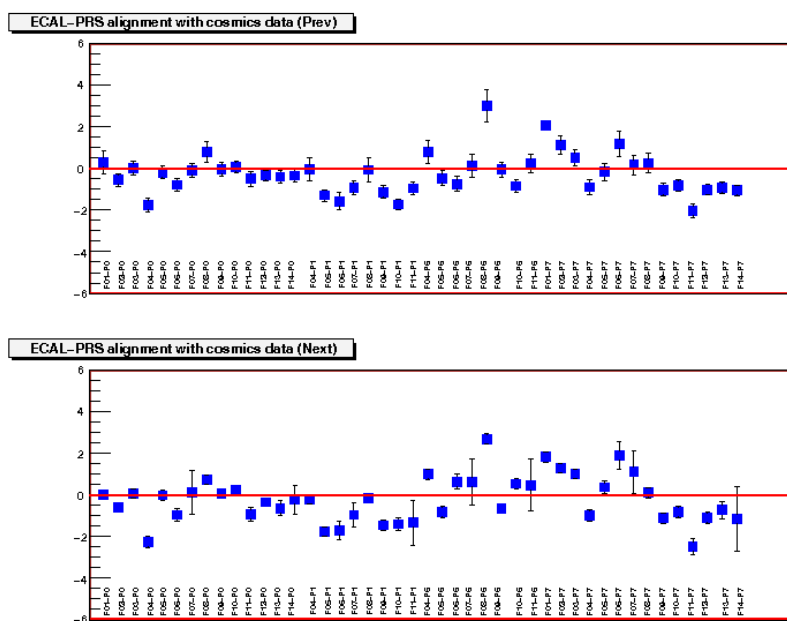
Figure 15 The measurements of the difference between the ECAL and PRS integration times, derived from asymmetry measurements. All the boards of the outer regions of the detector are displayed.
