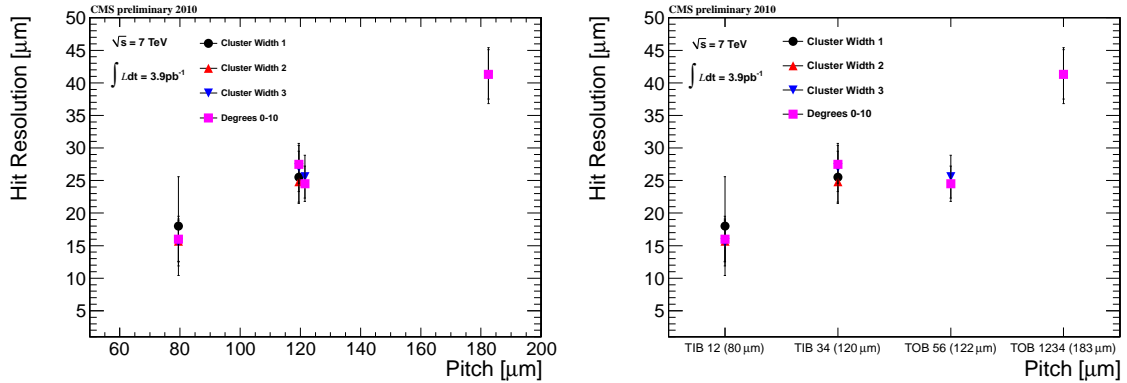
Figure 9: Detector hit resolutions measured using overlaps.
