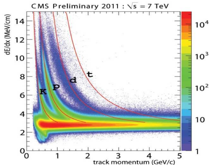
Figure 10: Measurement of dE/dx in the Silicon Strip Tracker.
